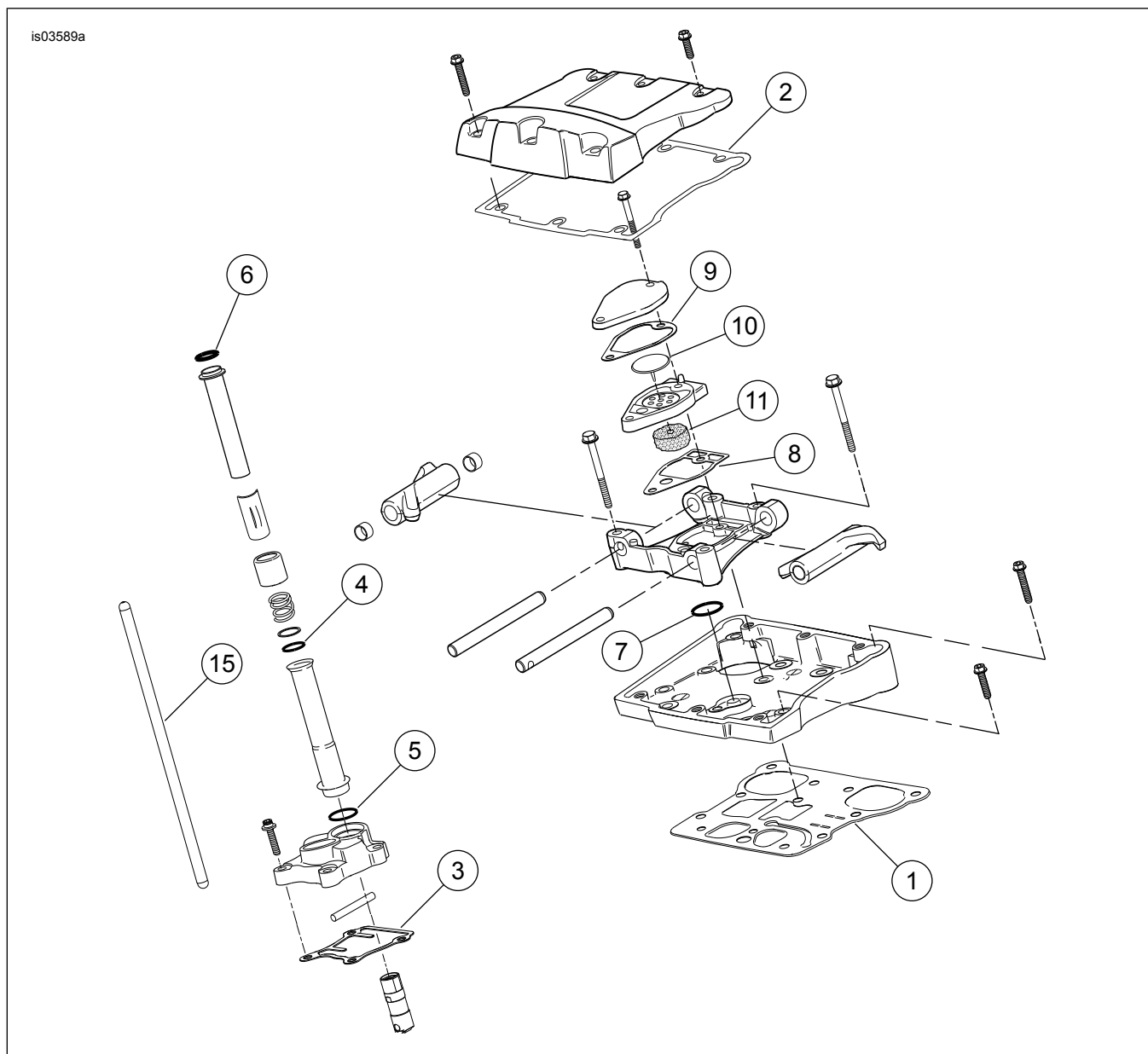
Figur 2. Reservdelar: Screamin' Eagle Pro TC 103 (1690 cc) Stage 4 Kit
