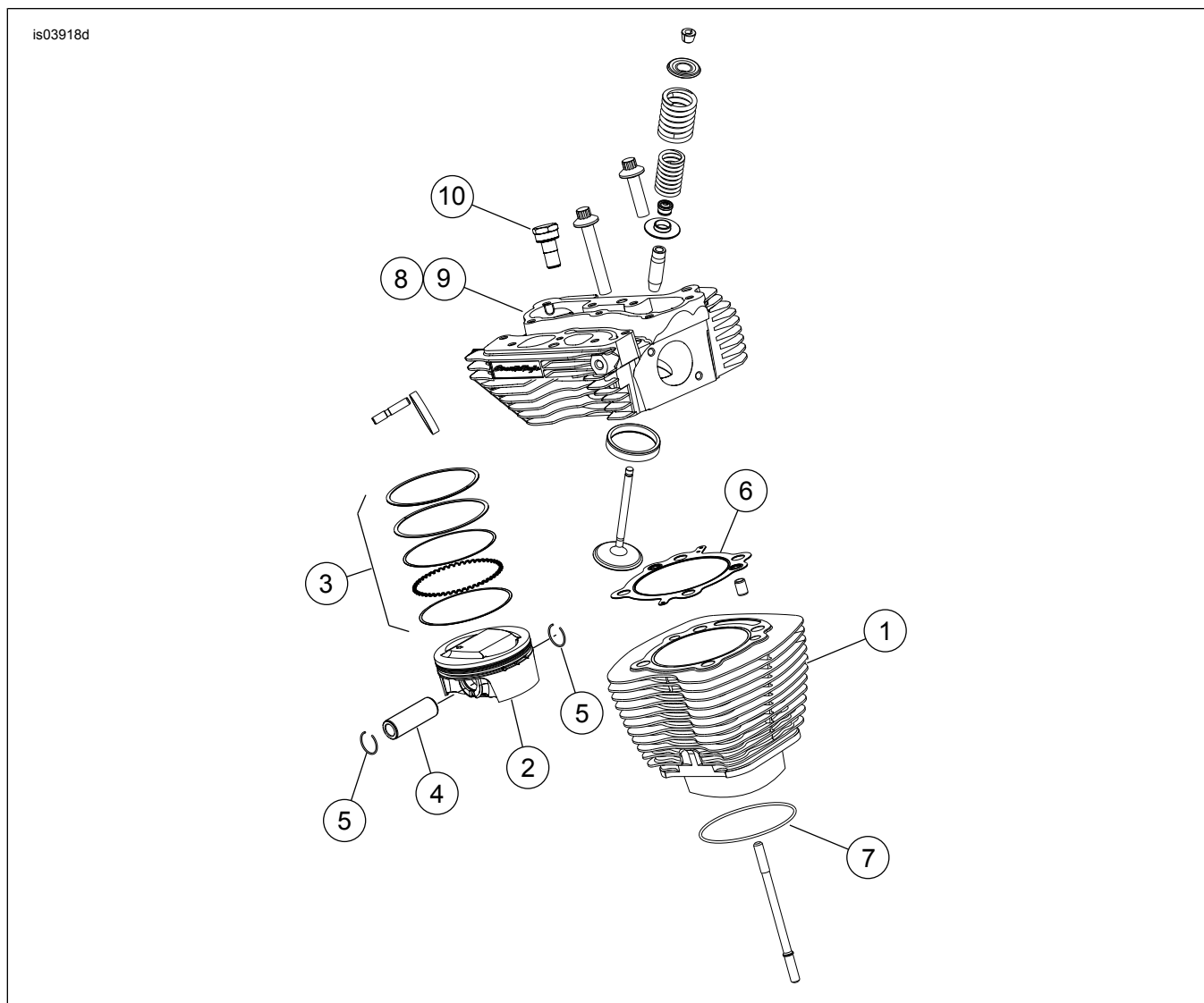
Figur 1. Reservdelar: Screamin' Eagle Pro TC 103 (1690 cc) Stage 4 Kit
