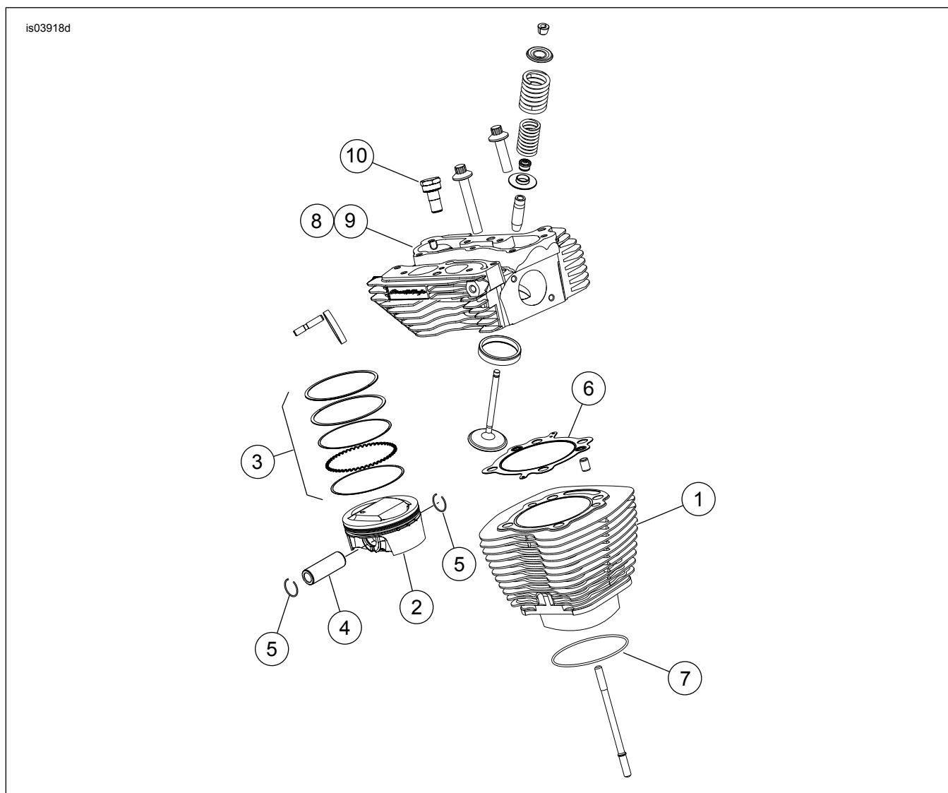
Figur 1. Servicedeler: Screamin' Eagle Pro TC 103 (1690 cc) nviå 4-sett
