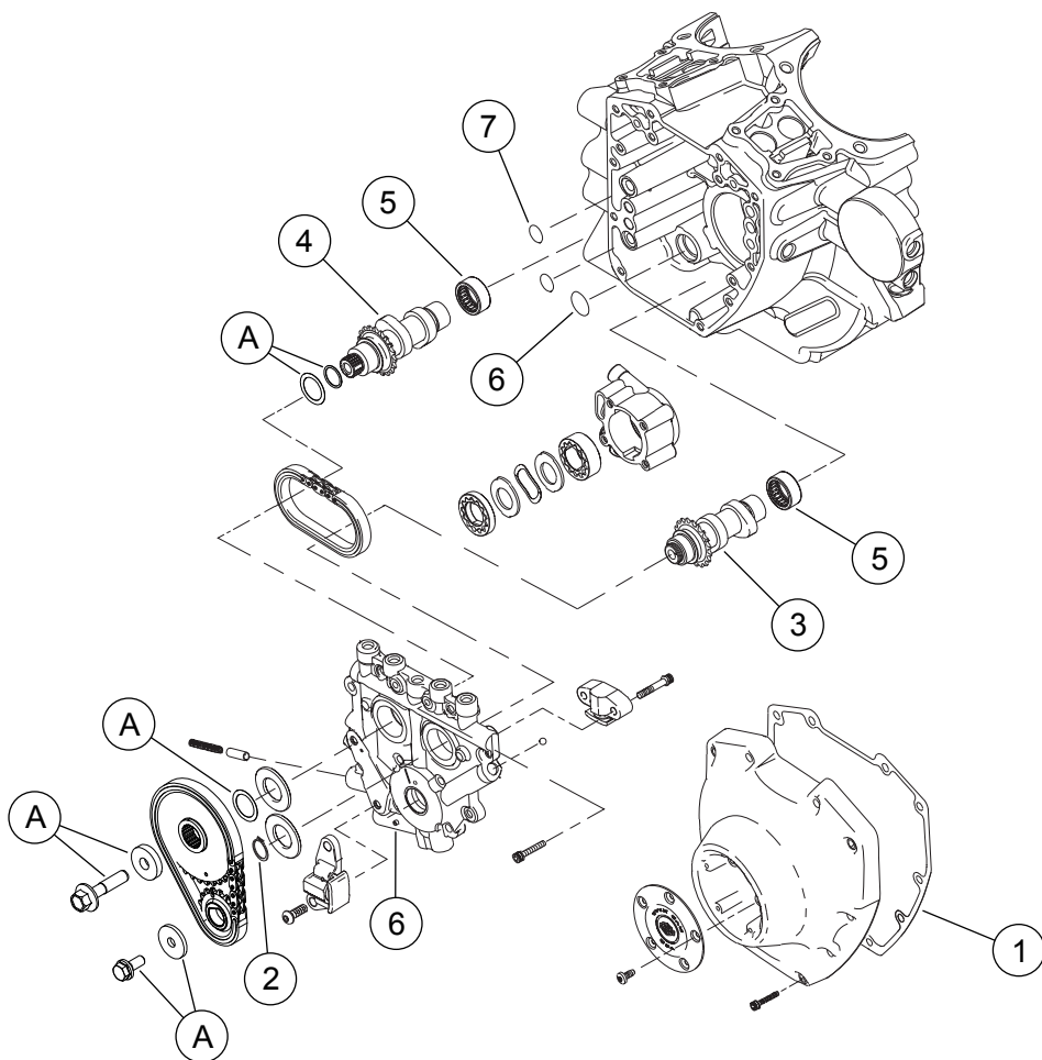
Figur 3. Servicedeler: Screamin' Eagle Pro TC 103 (1690 cc) nviå 4-sett
