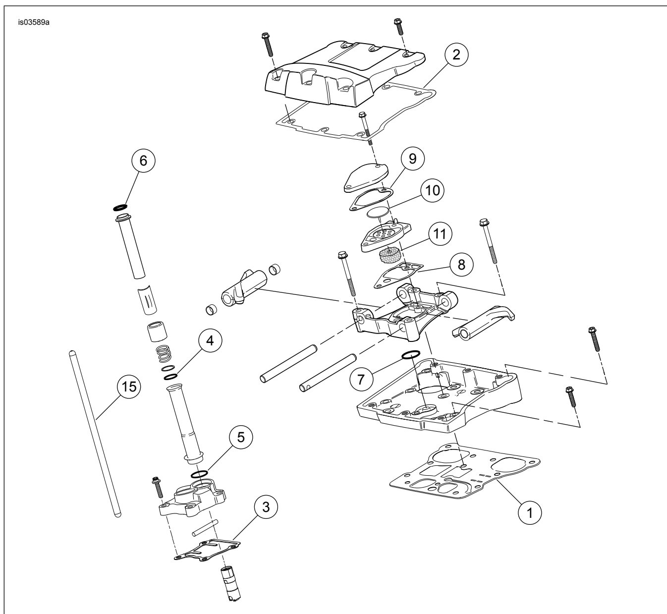
Figur 2. Reservedele: Screamin' Eagle Pro TC 103 (1690 cc) Stage 4 Kit
