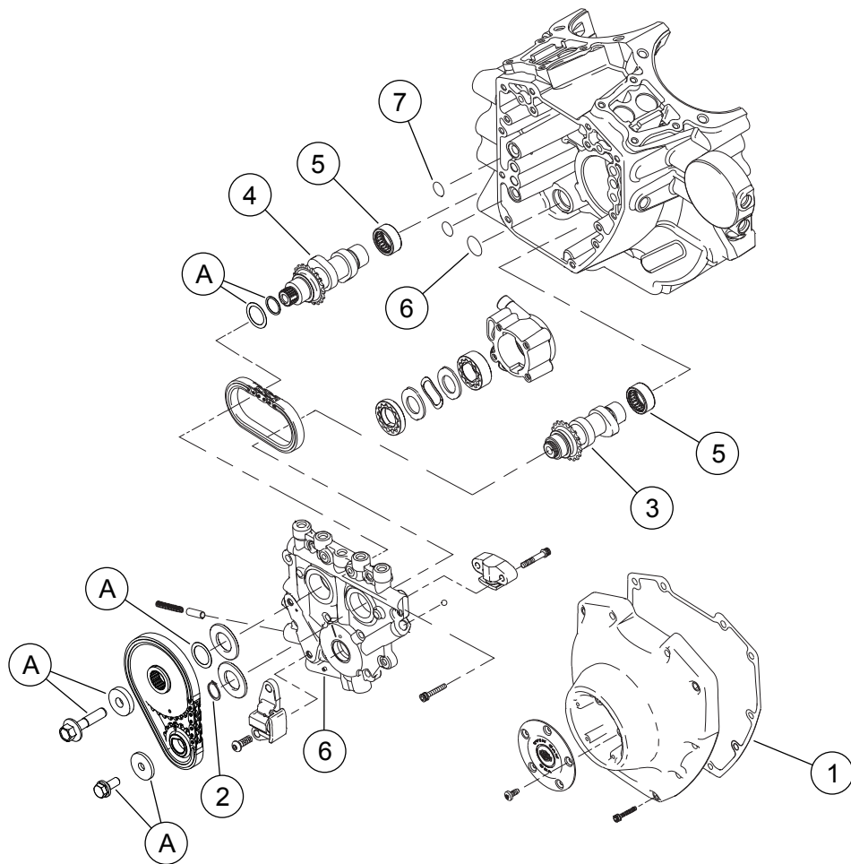
Figur 3. Reservedele: Screamin' Eagle Pro TC 103 (1690 cc) Stage 4 Kit
