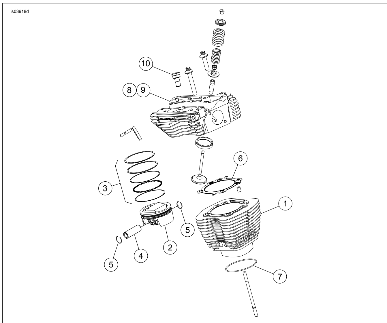
Figur 1. Reservedele: Screamin' Eagle Pro TC 103 (1690 cc) Stage 4 Kit
