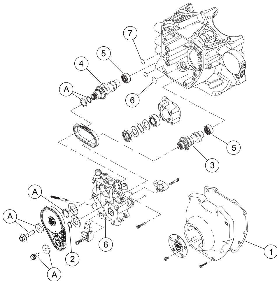
Figur 3. Reservdelar: Screamin' Eagle Pro TC (96 ci till 103 ci) Stage 4 Kit
