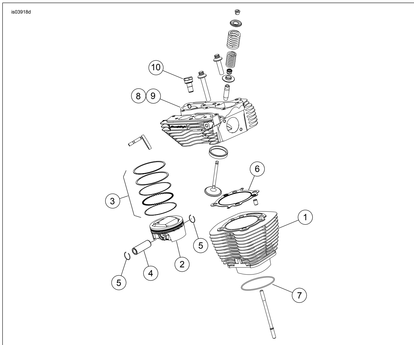
Figur 1. Reservdelar: Screamin' Eagle Pro TC (96 ci till 103 ci) Stage 4 Kit
