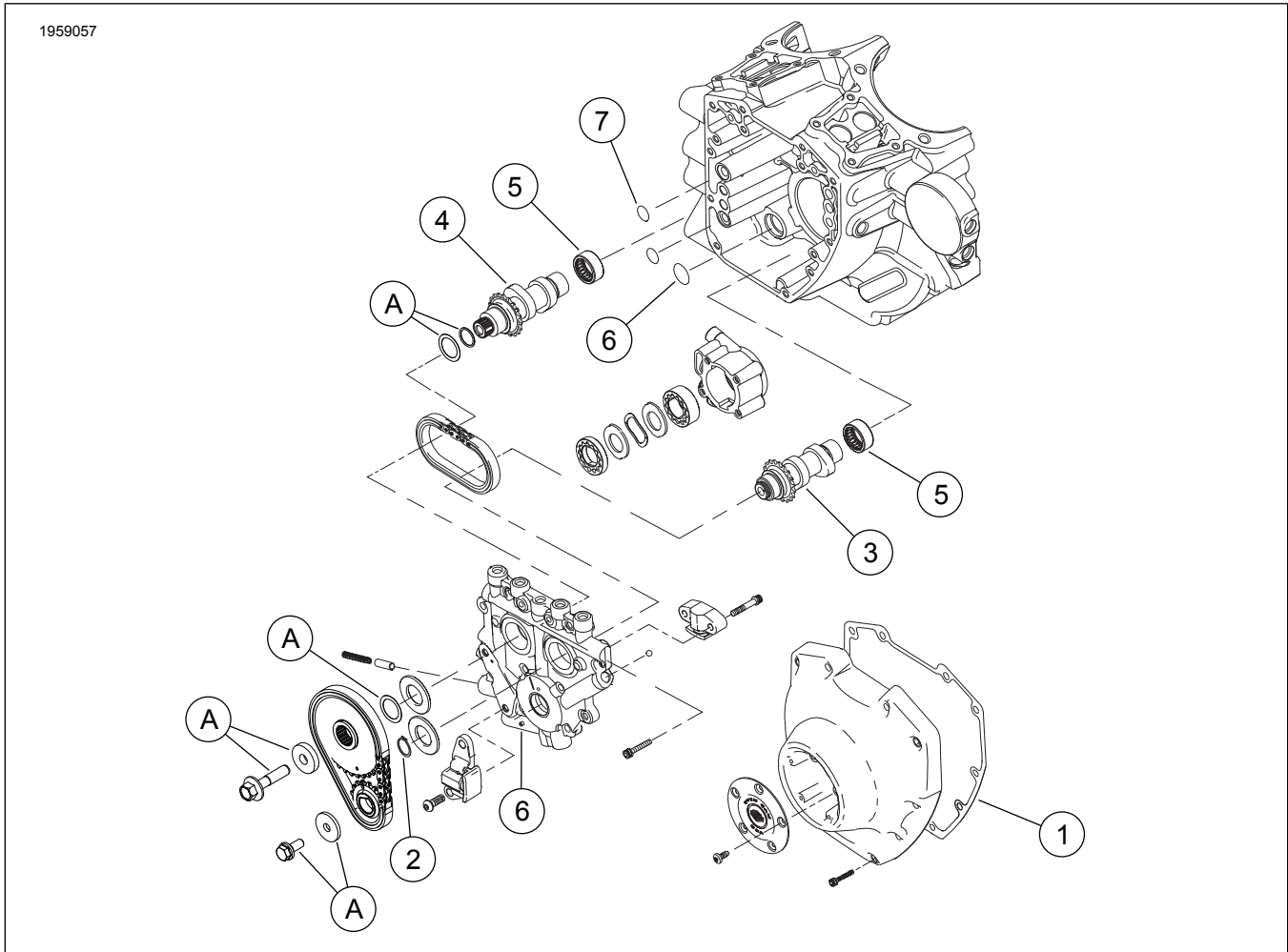
Gambar 3. Komponen Servis: Kit Screamin' Eagle Pro TC (96 ci hingga 103 ci) Stage 4
