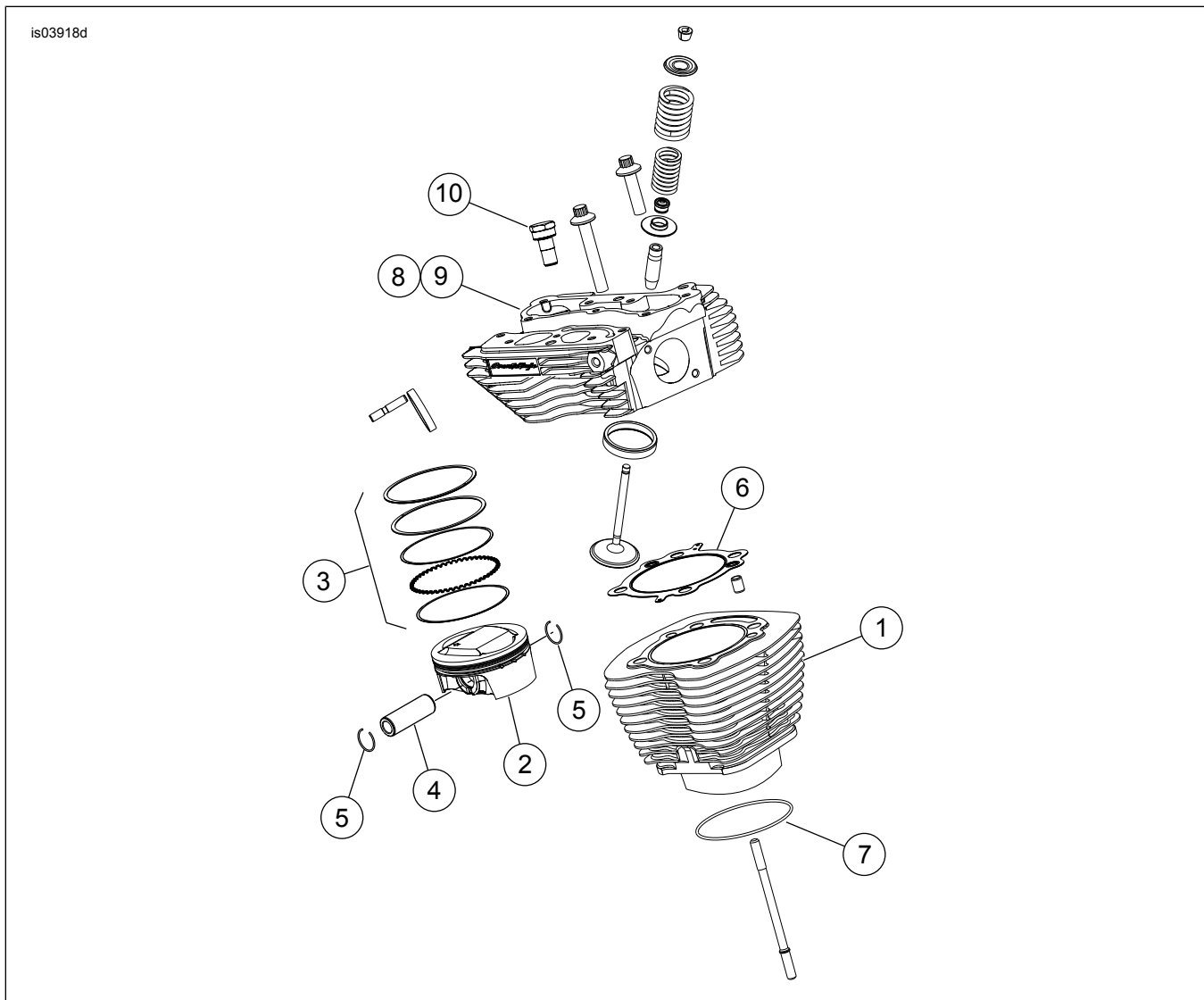
Gambar 1. Komponen Servis: Kit Screamin' Eagle Pro TC (96 ci hingga 103 ci) Stage 4
