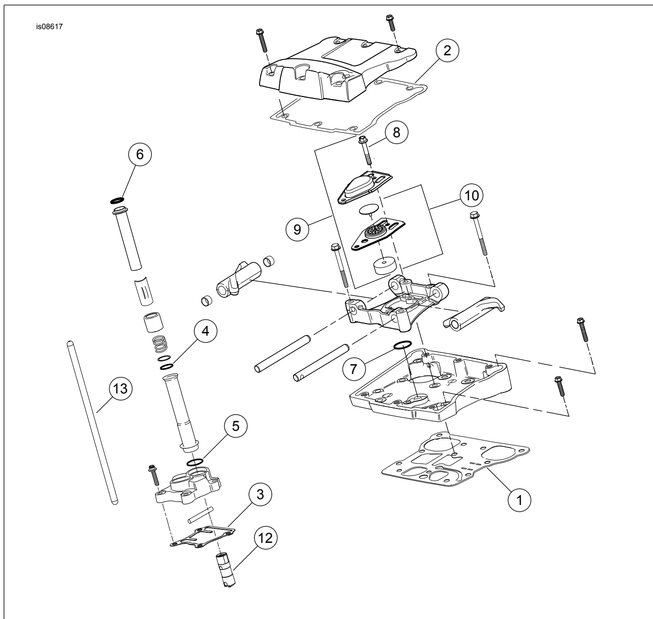
Figur 2. Reservedele: Screamin' Eagle Twin Cam 117 (1616 cc) Bolt-on Race Kit
