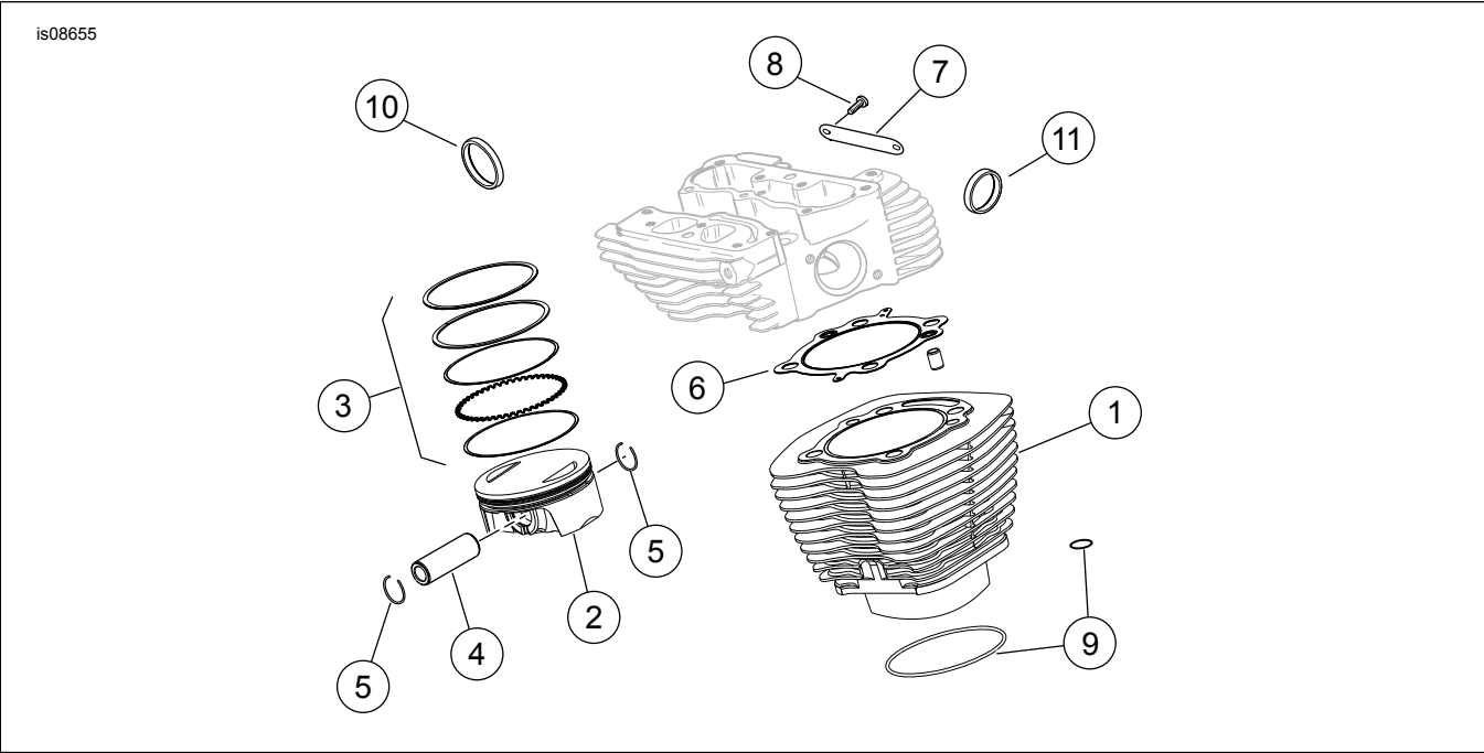
Figur 1. Reservedele: Screamin' Eagle Twin Cam 117 (1916 cc) Bolt-on Race Kit
