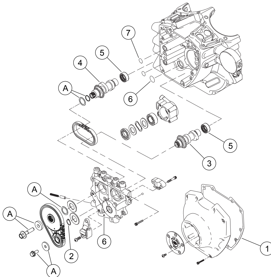
Figur 3. Servicedeler: Screamin' Eagle Pro 103 (1690 cc) nivå 4-sett
