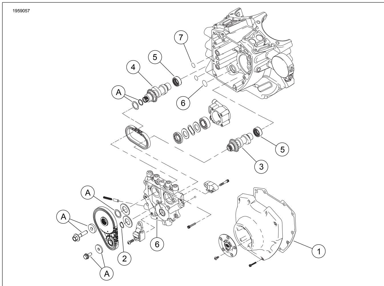
Figur 3. Reservedele: Screamin' Eagle Pro 103 (1690 cc) Stage 4 sæt
