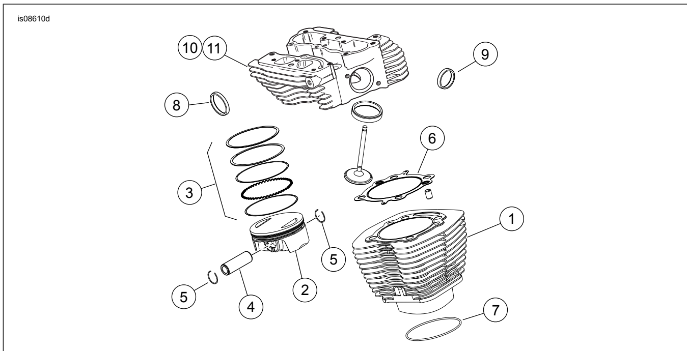
Figure 1. Mga Pamalit na Piyesa: Screamin' Eagle Twin Cam 110 (1800 cc) Stage V Race Kit
