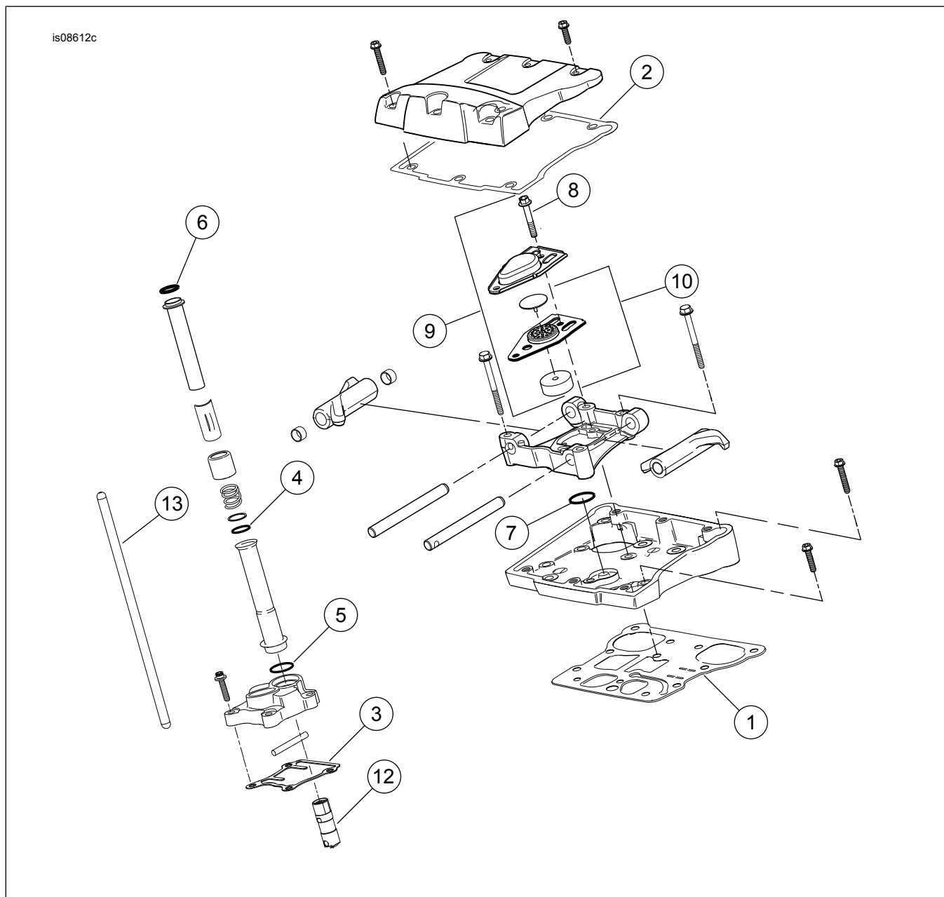
Figure 2. Mga Pamalit na Piyesa: Screamin' Eagle Twin Cam 110 (1800 cc) Stage V Race Kit
