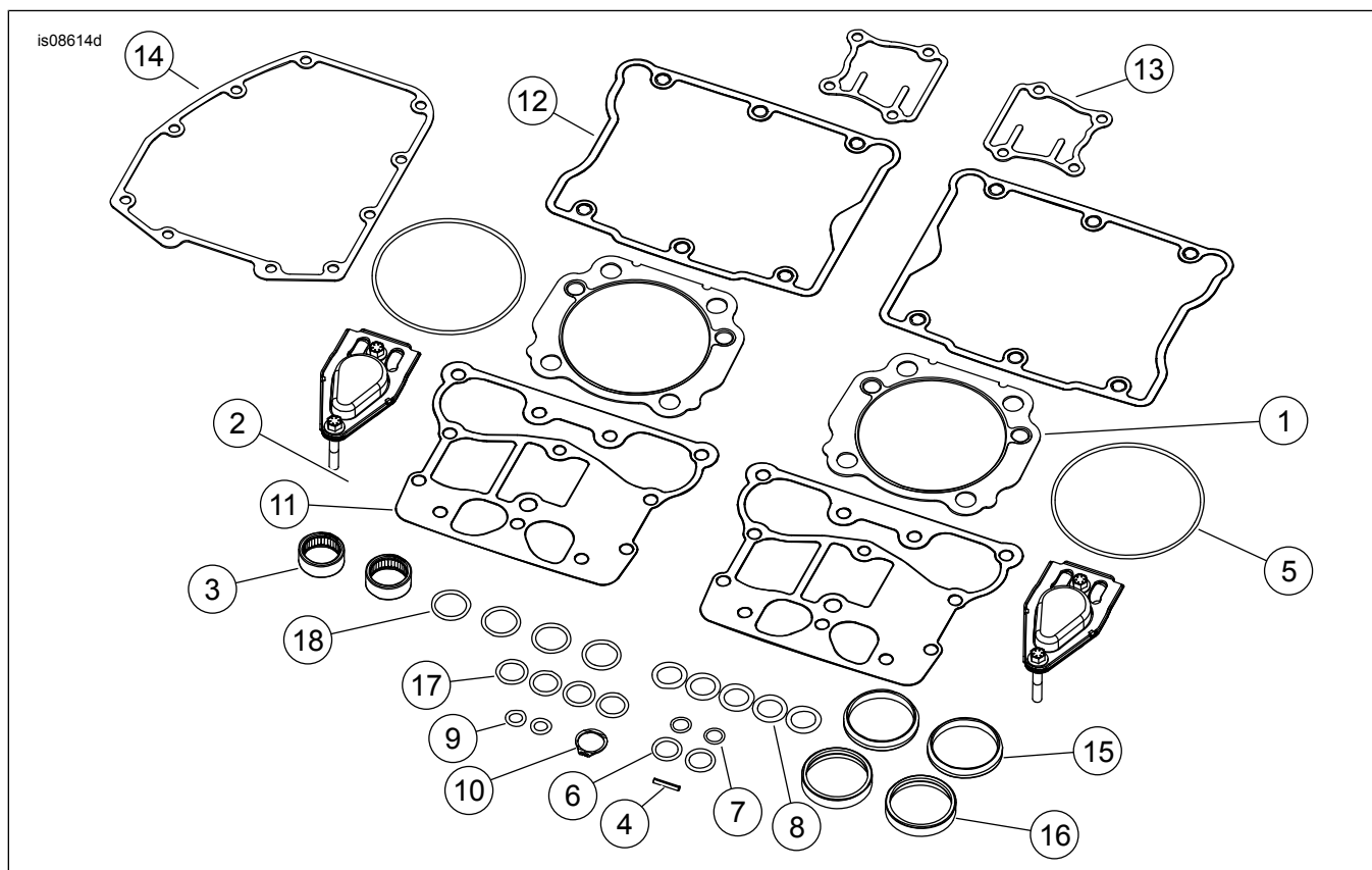
Figure 4. Mga Pamalit na Piyesa: Screamin' Eagle Twin Cam 110 (1800 cc) Stage V Race Kit
