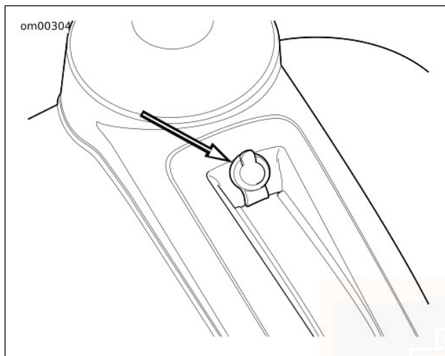
Figure 30. Front Headset Socket Cap VOX MICROPHONES
