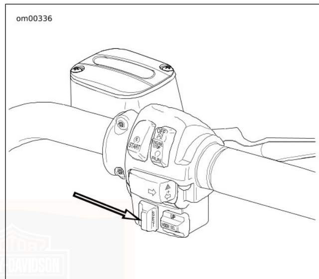
Figure 9. RESUME/SET Switch
