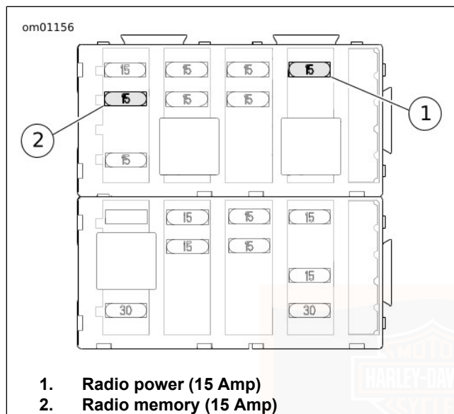
Figure 35. Radio Fuses
