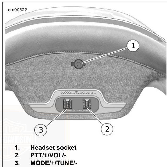
Figure 33. TLE Ultra Sidecar Audio Controls
