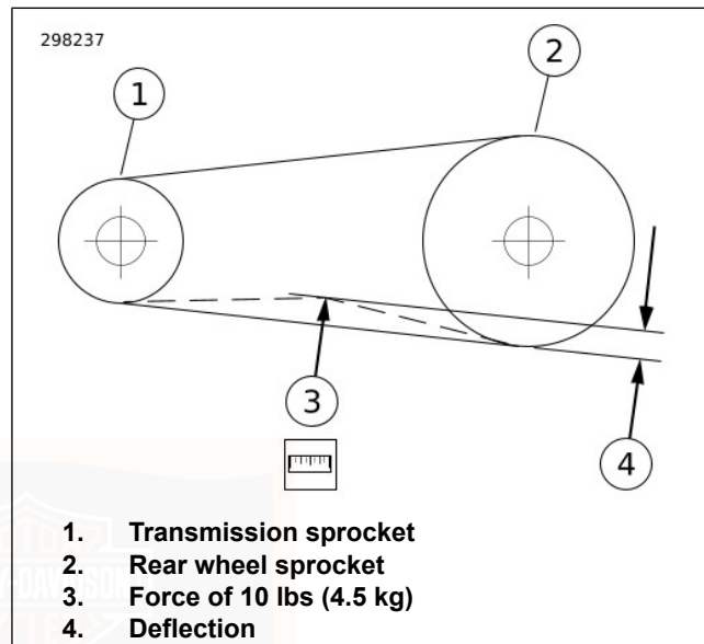
Figure 56. Check Belt Deflection
