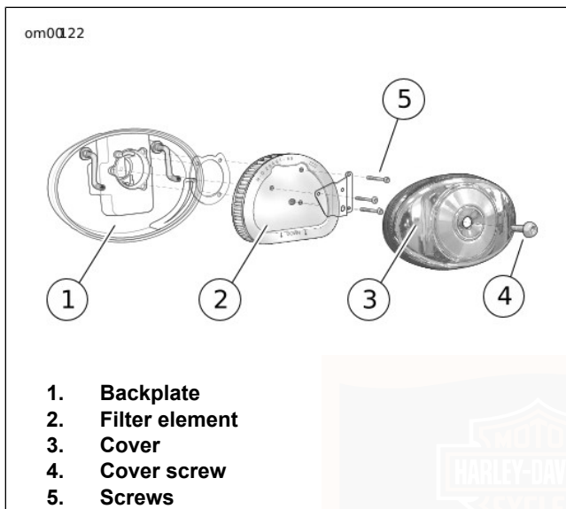
Figure 60. Air Cleaner: Twin Cam Models
