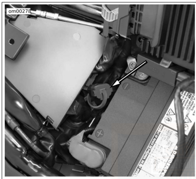
Figure 21. Accessory Connector
