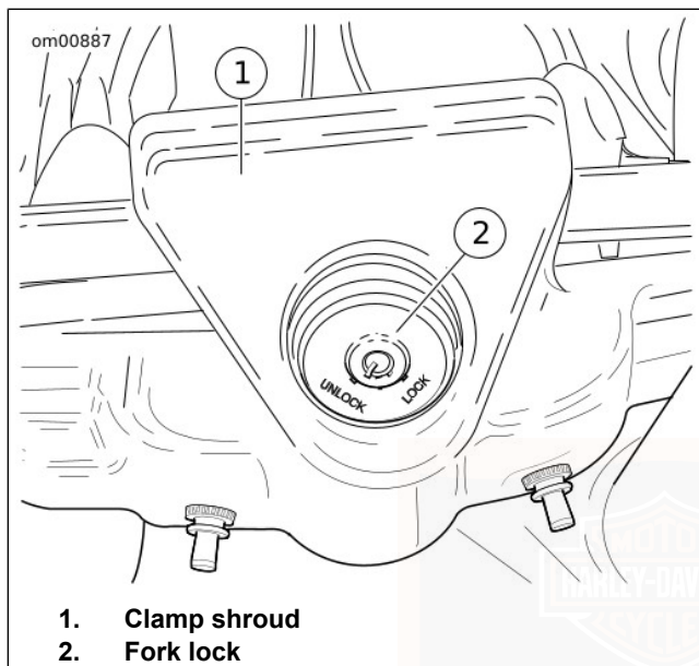
Figure 4. Fork Lock: FLHR/FLHRC HAND CONTROLS: BASIC OPERATION
