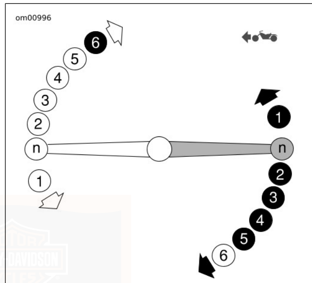
Figure 48. Heel-Toe Foot Shift Lever
