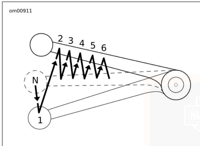
Figure 46. Shifting Sequence: Upshift
