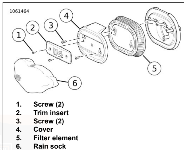
Figure 80. Air Cleaner: Oval
