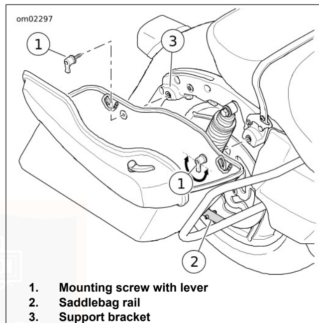
Figure 57. Saddlebag Removal/Installation
