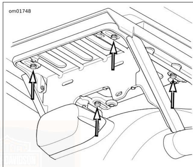
Figure 60. Tour-Pak Bracket Screws (APC Models)
