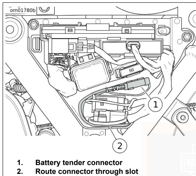
Figure 82. Battery Tender Connector (under left side cover)
