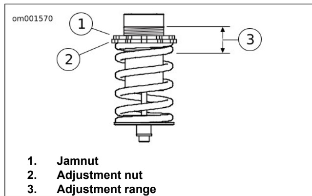
Figure 104. Seat Adjustment
