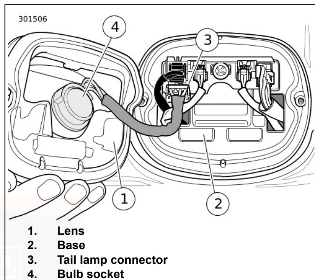
Figure 96. Tail Lamp Assembly
