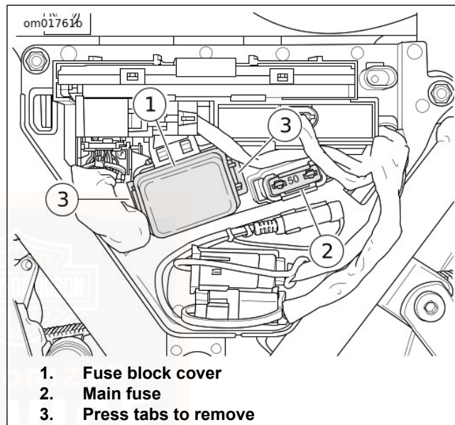
Figure 86. Fuse Block (under left side cover)
