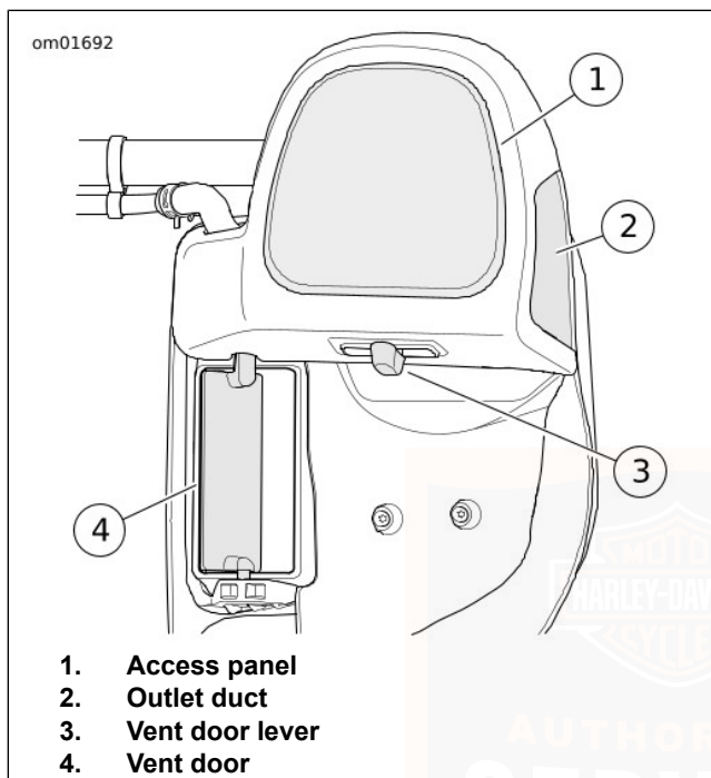
Figure 55. Fairing Lowers: Twin-Cooled Models
