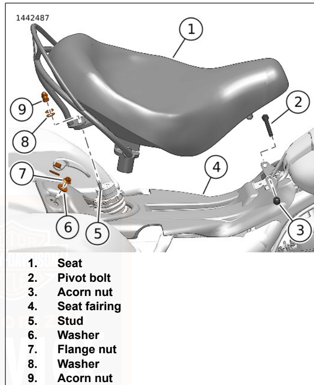
Figure 99. Seat Attachment (Spring mount)
