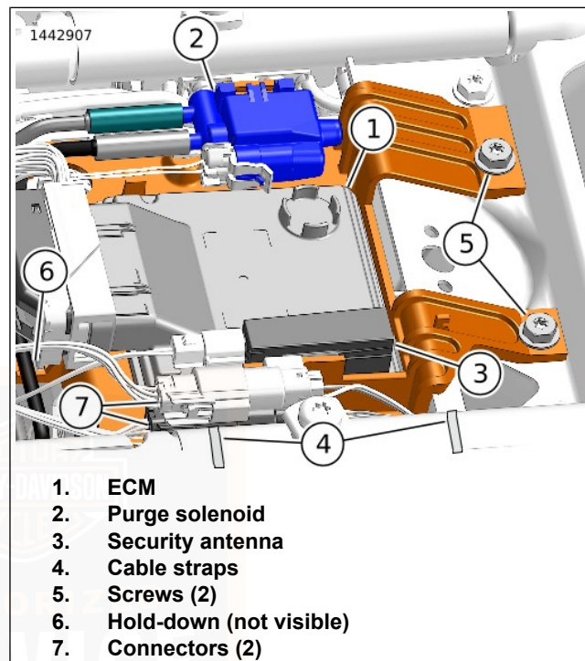
Figure 84. Top Caddy
