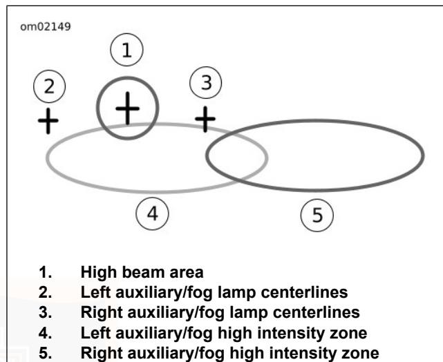
Figure 93. Headlamp Pattern: Quartz Halogen Type
