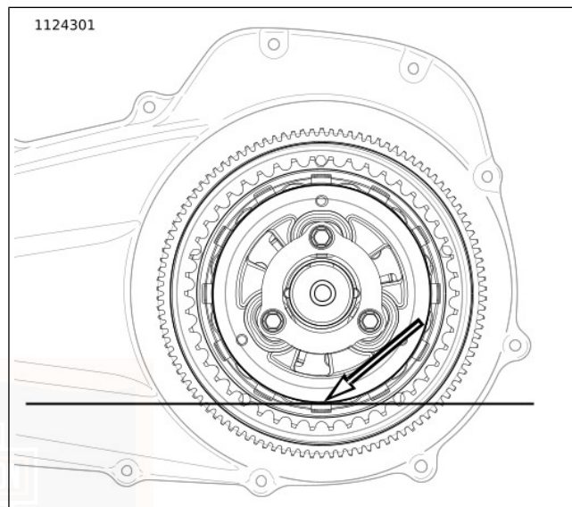
Figure 69. Primary Lubricant Level
