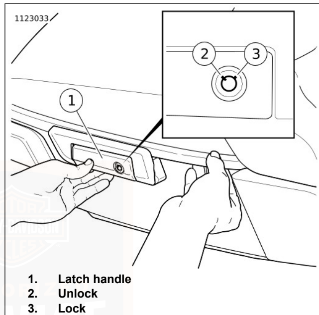
Figure 58. Tour-Pak
