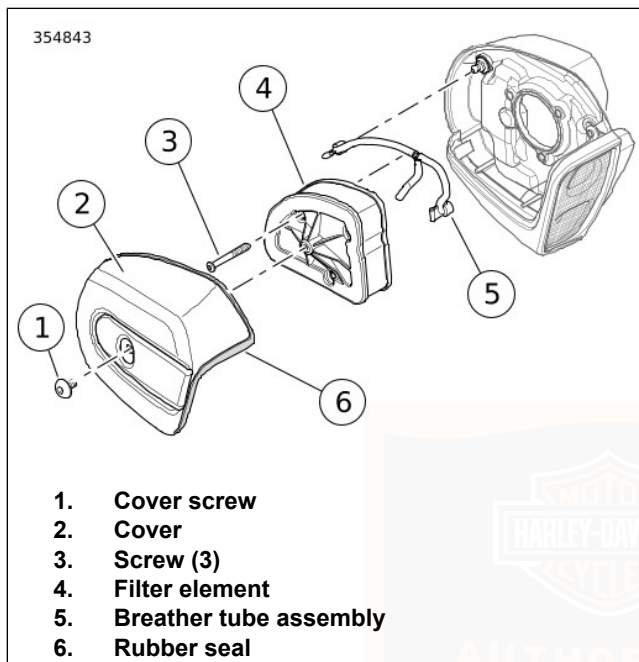
Figure 79. Air Cleaner Assembly (typical)
