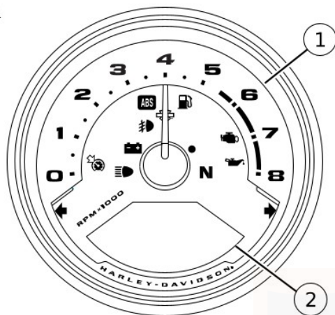
Figure 27. Instruments: Fat Bob 114 (FXFBS), Low Rider S (FXLRS)
