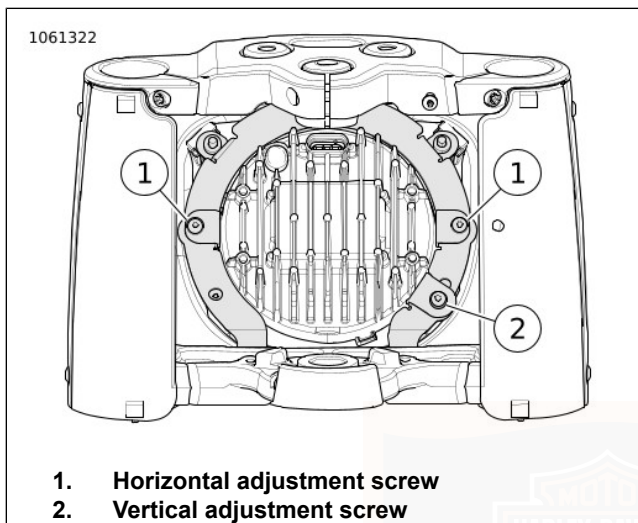
Figure 82. Headlamp Adjustment
