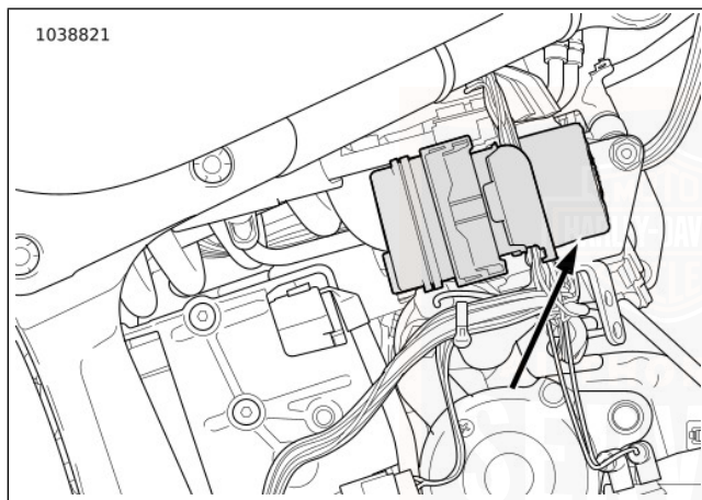
Figure 38. ABS Module (EHCU)
