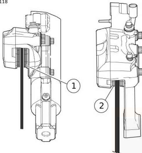
Figure 62. Brake Friction Material
