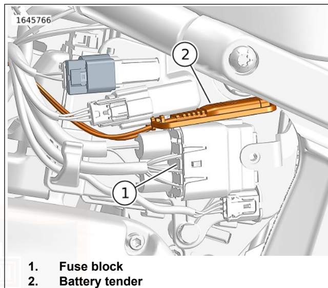
Figure 73. Fuses
