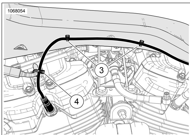
Figure 3. 10MM Spark Plug Wire Routing (left)
