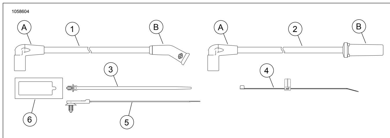
Figure 5. Service Parts: 10 MM Spark Plug Cables
