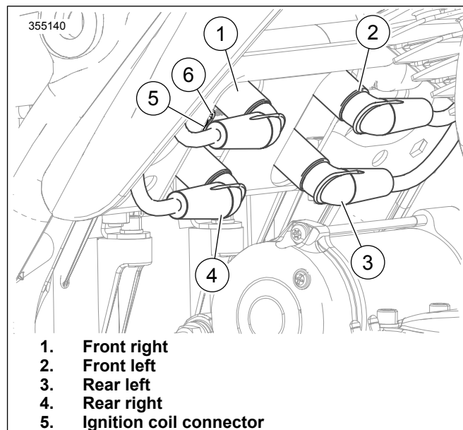
Figure 1. Coil Spark Plug Cables
