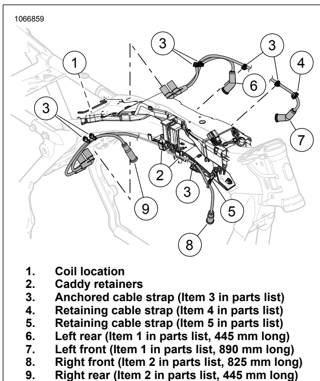
Figure 2. Motor Spark Plug Cables
