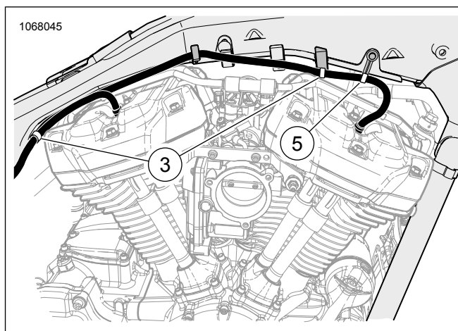
Figure 4. 10MM Spark Plug Wire Routing (right)
