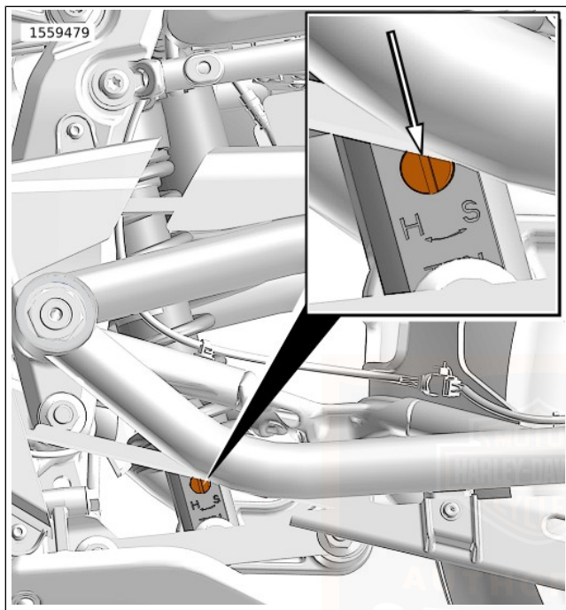
Figure 12. Rebound Adjuster
