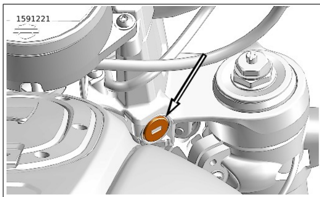
Figure 25. Fork Lock
