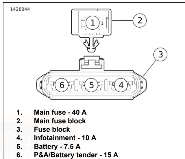
Figure 71. Fuse Blocks and Socket Terminals
