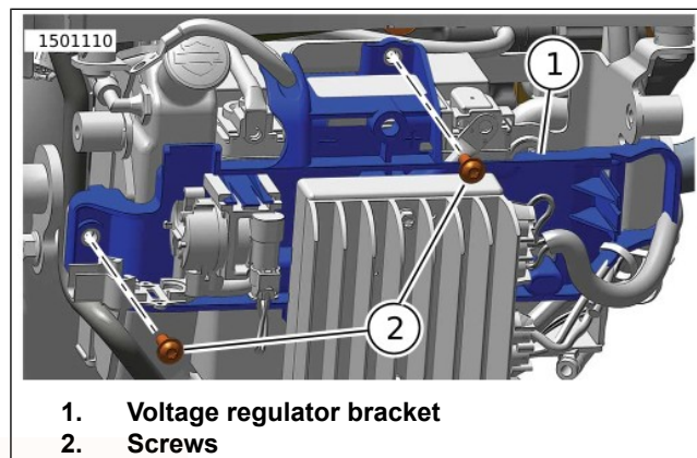
Figure 59. Voltage Regulator Bracket Screws
