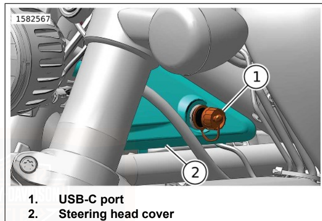
Figure 35. USB-C Port HEATED GEAR CONNECTOR
