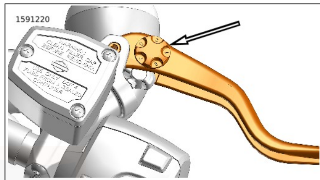
Figure 24. Brake Lever Adjustment Dial (Typical)
