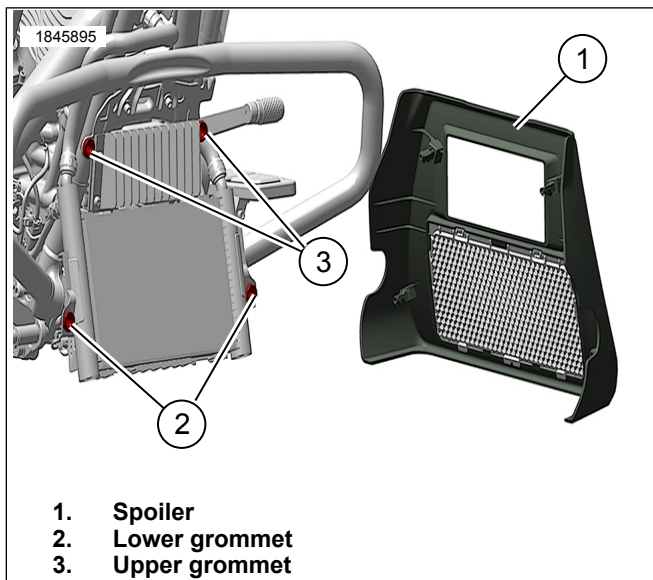
Figure 3. Chin spoiler
