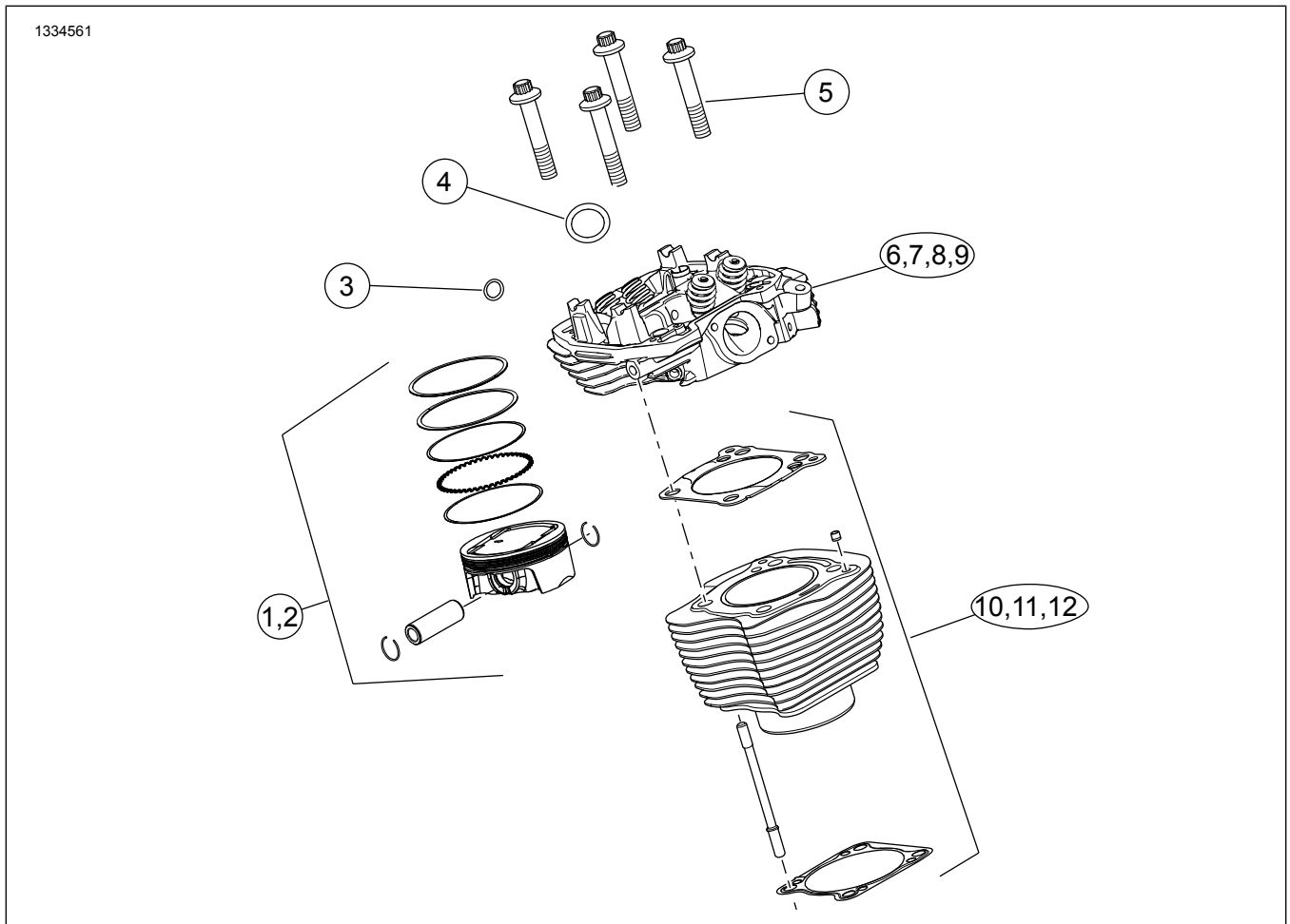
Figure 1. Kit Contents: Top End: Screamin' Eagle Milwaukee-Eight™ Stage IV Components
