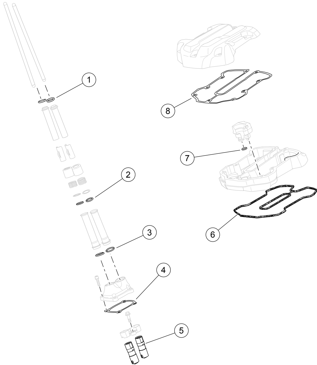
Figure 2. Kit Contents: Valve Train: Screamin' Eagle Milwaukee-Eight™ Stage IV Components
