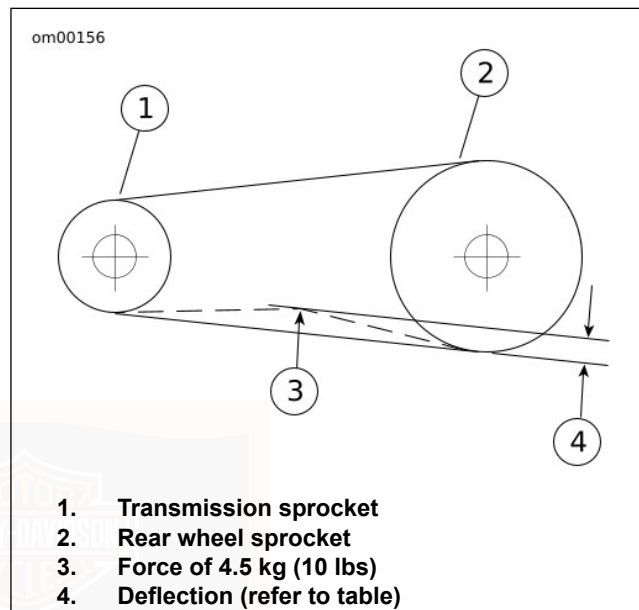
Figure 47. Check Belt Deflection: Sportster Models
