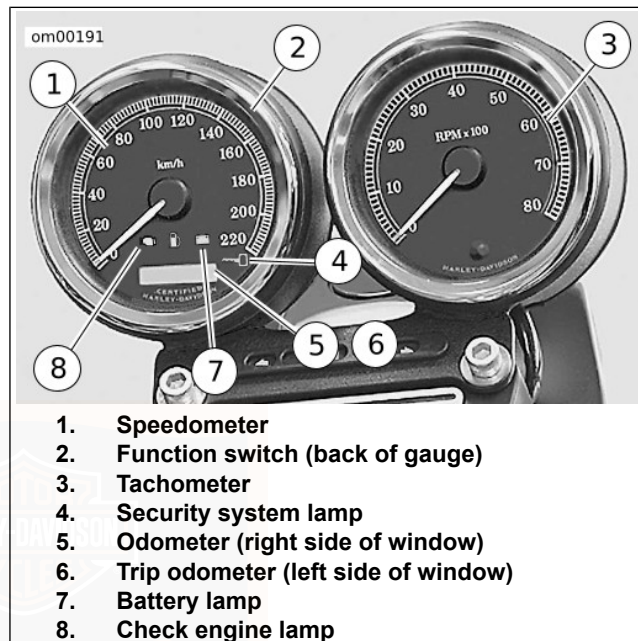
Figure 19. Speedometer/Odometer and Tachometer: International Sportster Models (1200R Roadster)
