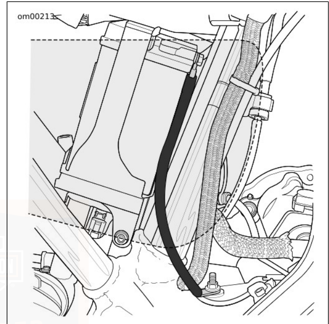
Figure 59. Negative Battery Cable and Crankcase Stud: Sportster Models
