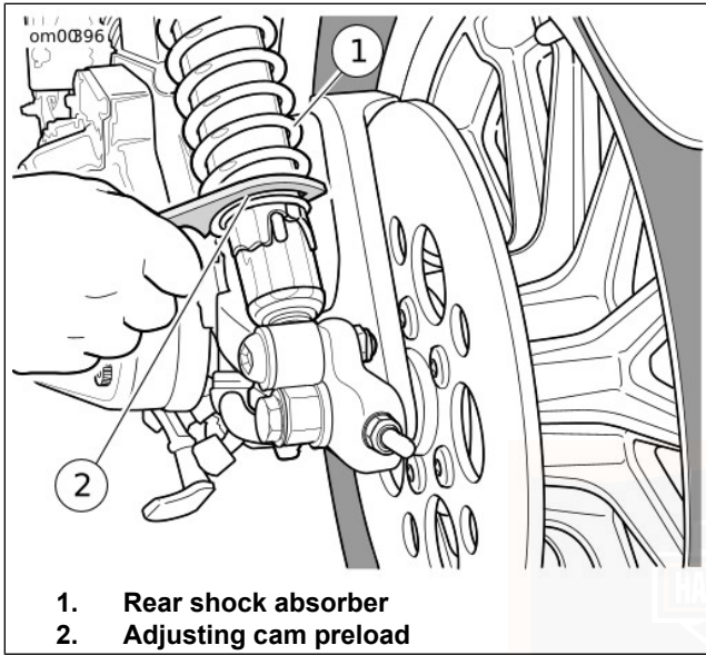
Figure 27. Rear Shock Absorber Adjustment: Sportster Models
