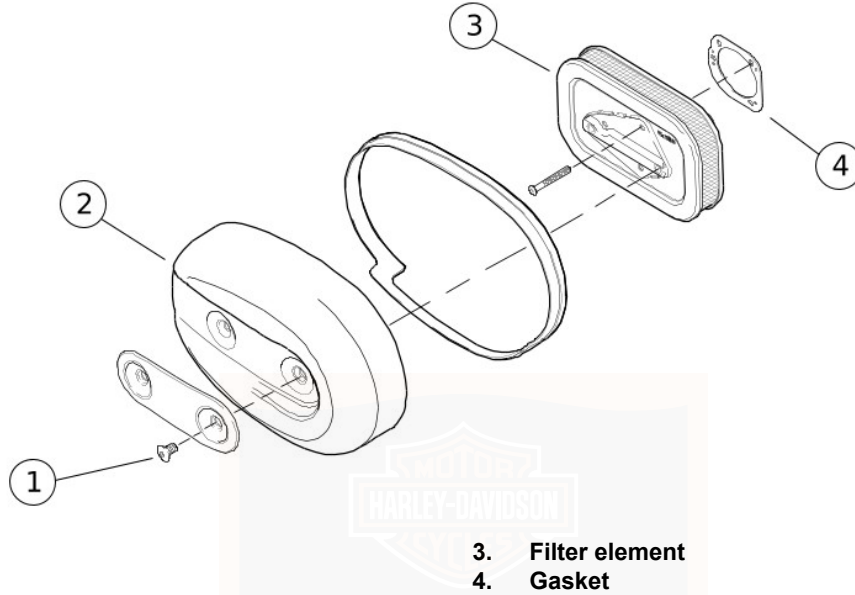
Figure 50. Air Cleaner Assembly: Sportster Models
