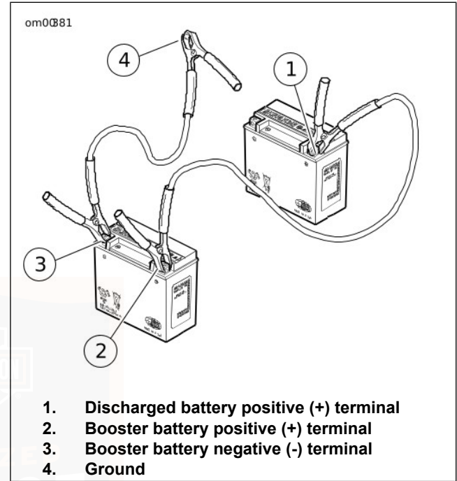
Figure 60. Jump Start Cable Connections
