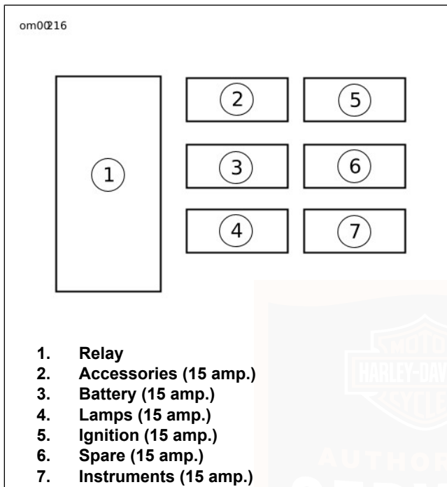
Figure 62. Fuse Block: Sportster Models
