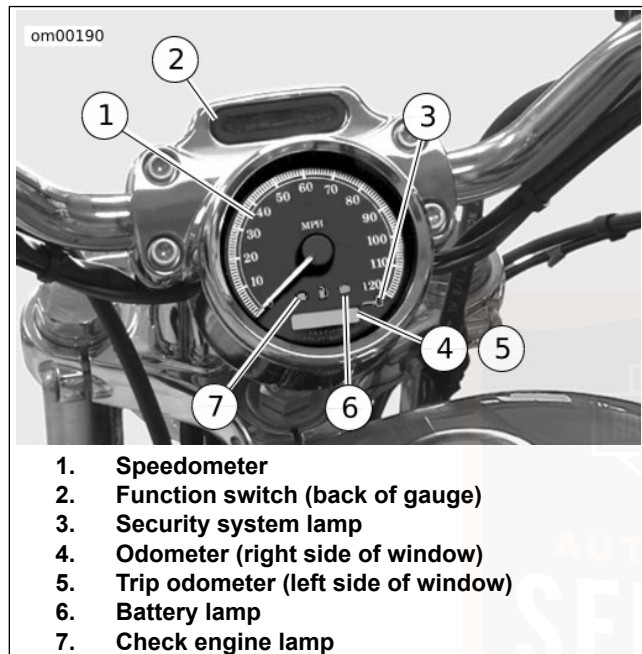
Figure 18. Speedometer/Odometer: Sportster Models (1200 Custom)
