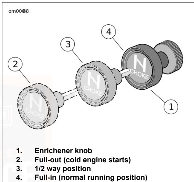
Figure 20. Setting the Enrichener
