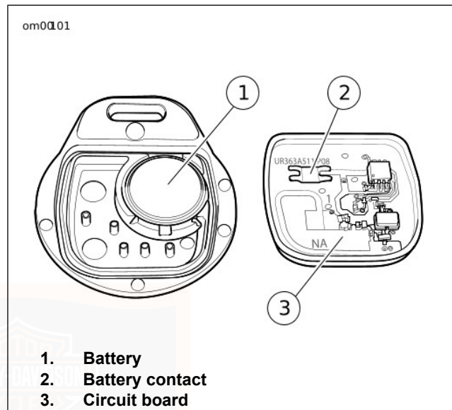
Figure 33. Key Fob Battery Replacement
