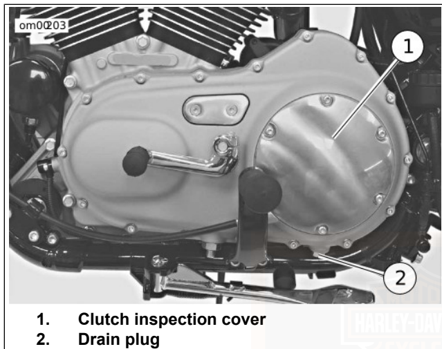
Figure 43. Primary Cover: Sportster Models
