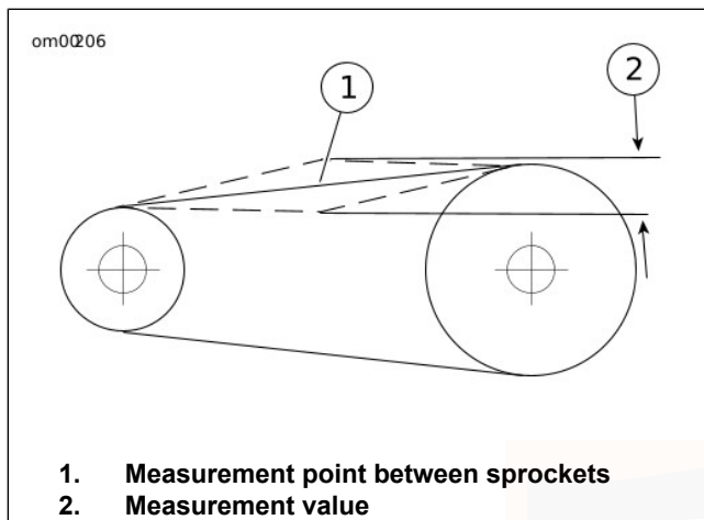
Figure 45. Primary Chain Vertical Free Play: Sportster Models
