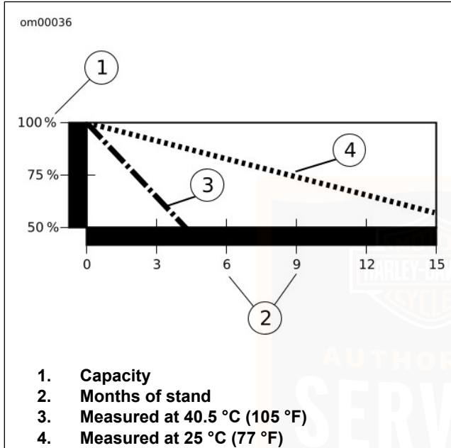
Figure 58. Effective Rate of Temperature on Battery Self-discharging Rate
