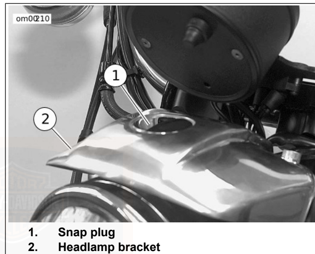
Figure 53. Headlamp Snap Plug: Sportster Models
