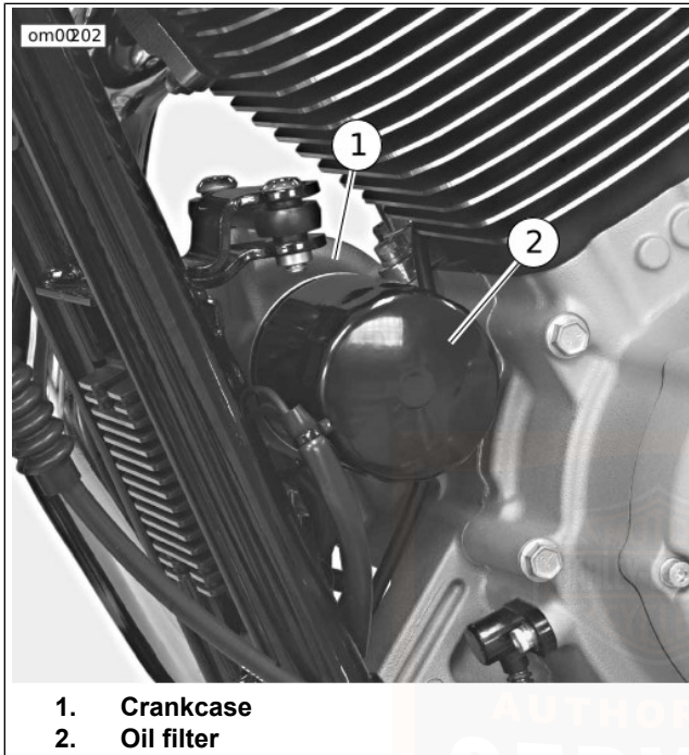
Figure 40. Oil Filter: Sportster Models
