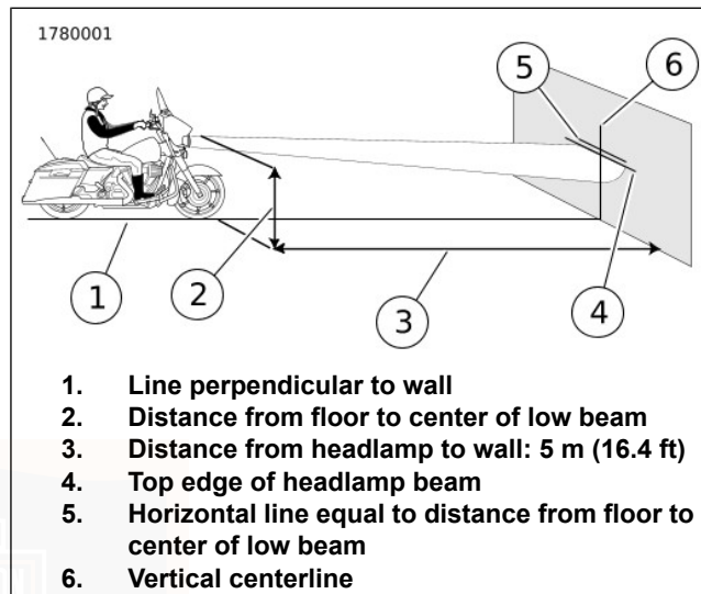
Figure 122. Headlamp Alignment
