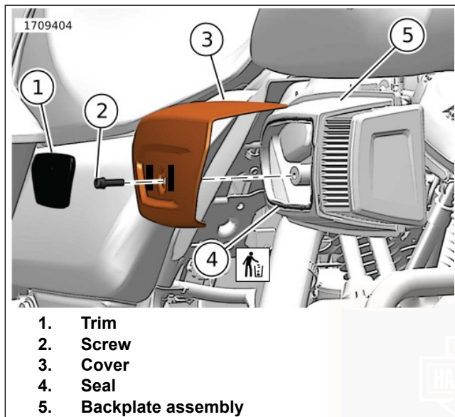
Figure 108. Air Cleaner Cover
