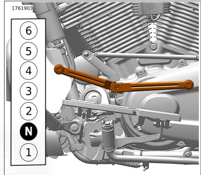
Figure 25. Gear Shift Lever and Shift Pattern
