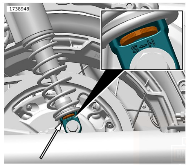
Figure 15. Damping Adjustment Thumbwheel (Both Shock Absorbers)
