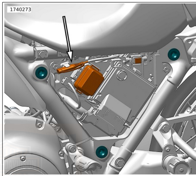
Figure 112. Battery Tender Connector (under left side cover)
