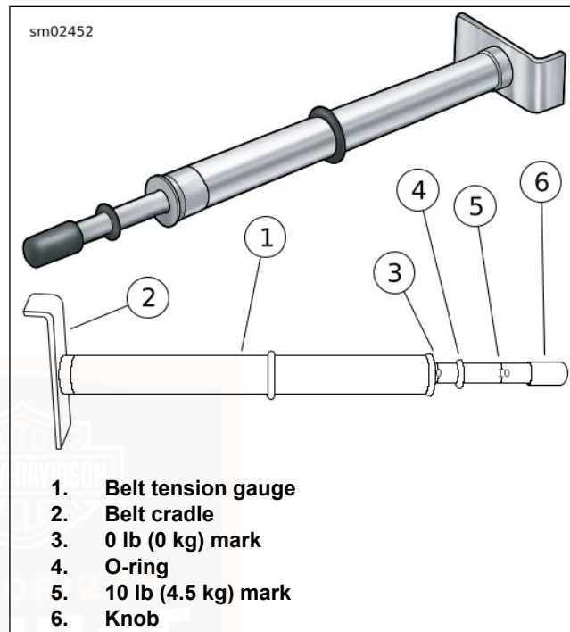
Figure 105. Belt Tension Gauge
