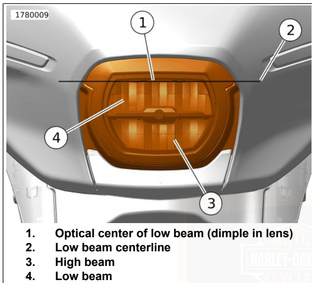
Figure 121. Headlamp Components
