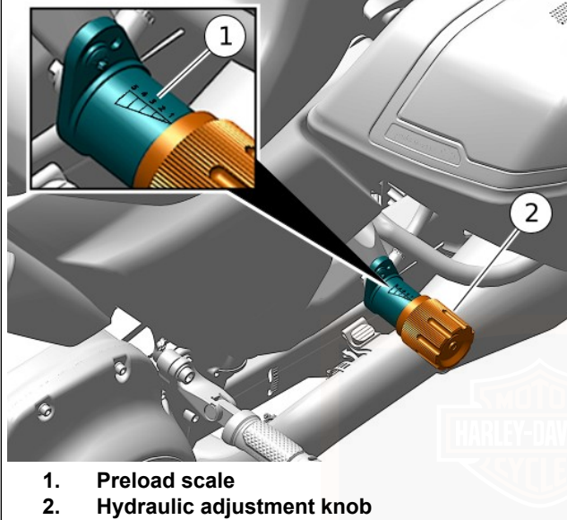
Figure 14. Hydraulic Preload Adjustment Knob (Left Side Shock Absorber)
