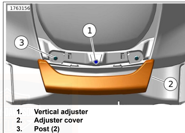
Figure 124. Headlamp Adjustment HEADLAMP REPLACEMENT
