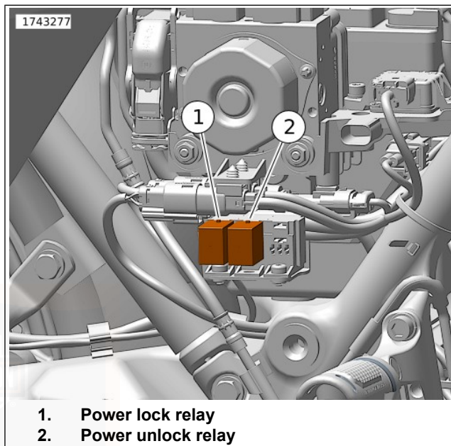
Figure 120. Power Lock Relays (under right side cover)
