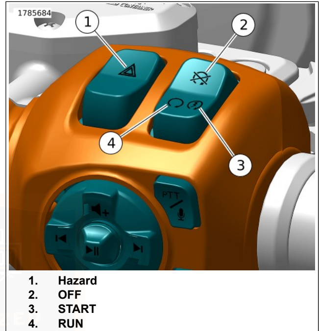
Figure 60. RHCM: OFF/RUN/START and Hazard Buttons
