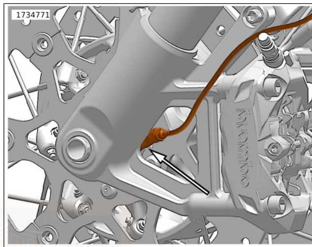
Figure 9. Wheel Speed Sensor (ABS identification typical)
