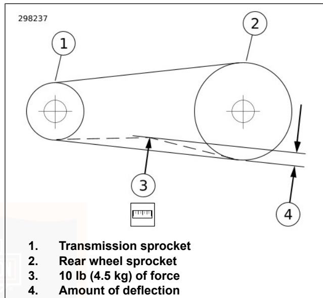
Figure 107. Checking Belt Deflection
