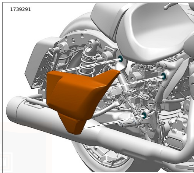
Figure 111. Side Cover BATTERY TENDER CONNECTOR
