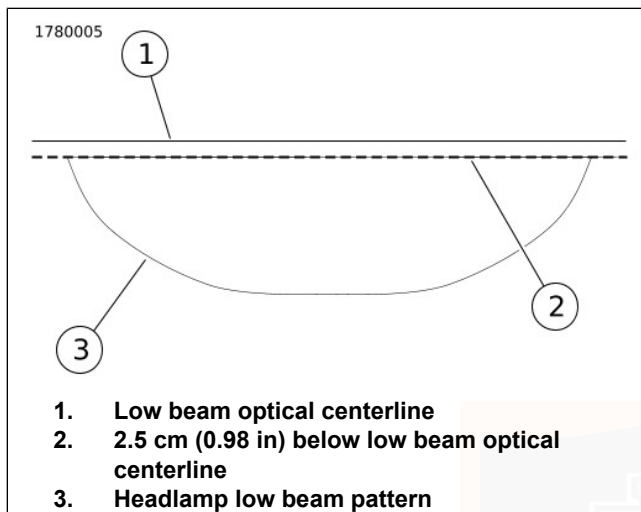
Figure 123. Alignment of Headlamp Low Beam
