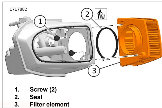
Figure 109. Air Filter Element
