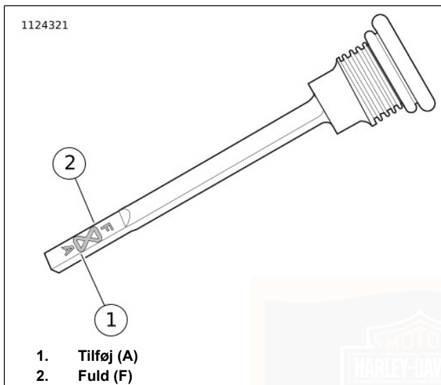
Figur 51. Smøreoliestand i transmission SKIFT TRANSMISSIONSSMØREOLIE
