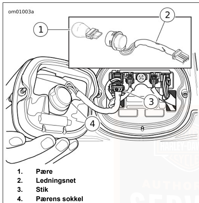
Figur 86. Baglys
