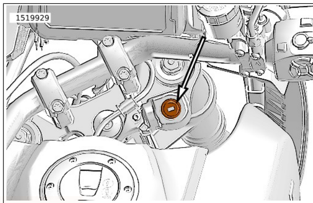
Figure 30. Fork Lock
