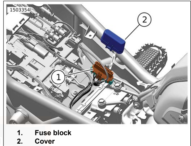
Figure 87. Fuse Block - Location
