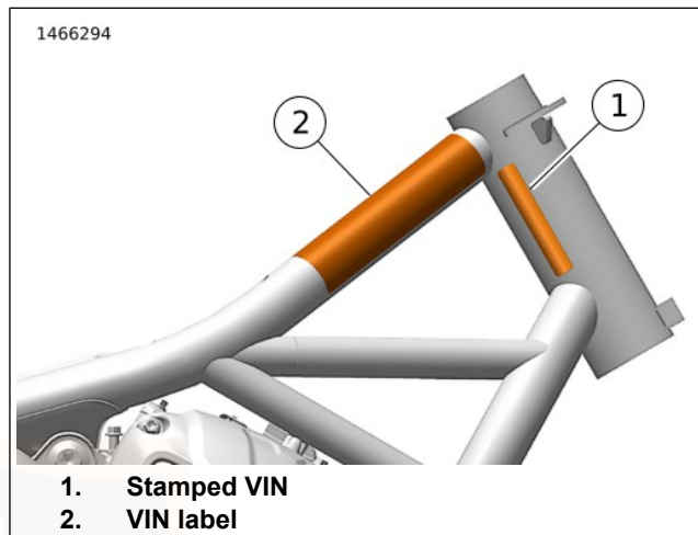
Figure 2. VIN Locations
