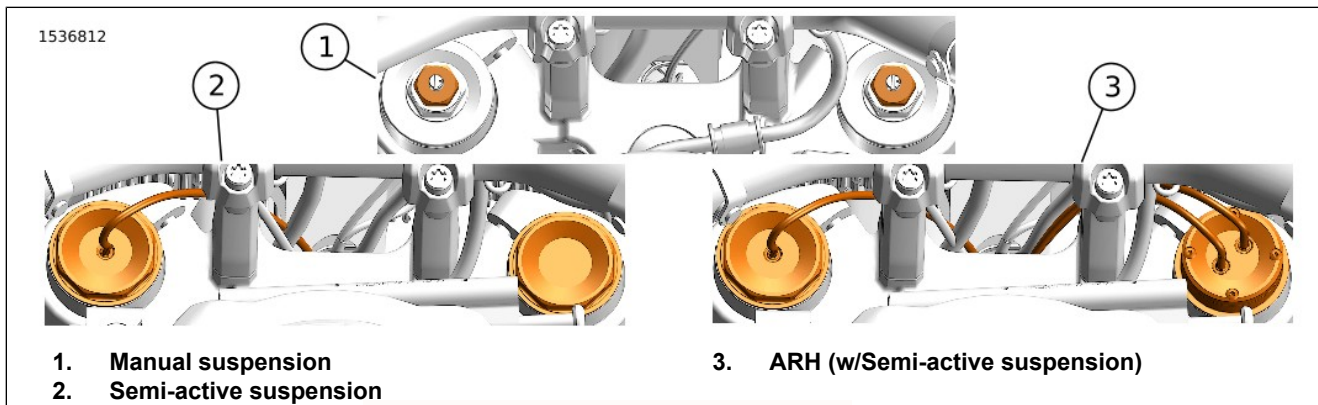
Figure 12. Front Suspensions
