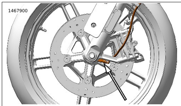
Figure 9. Wheel Speed Sensor (ABS identification)
