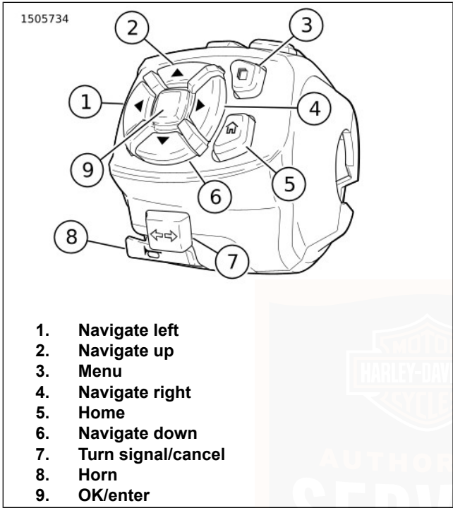
Figure 35. LHCM - Bottom
