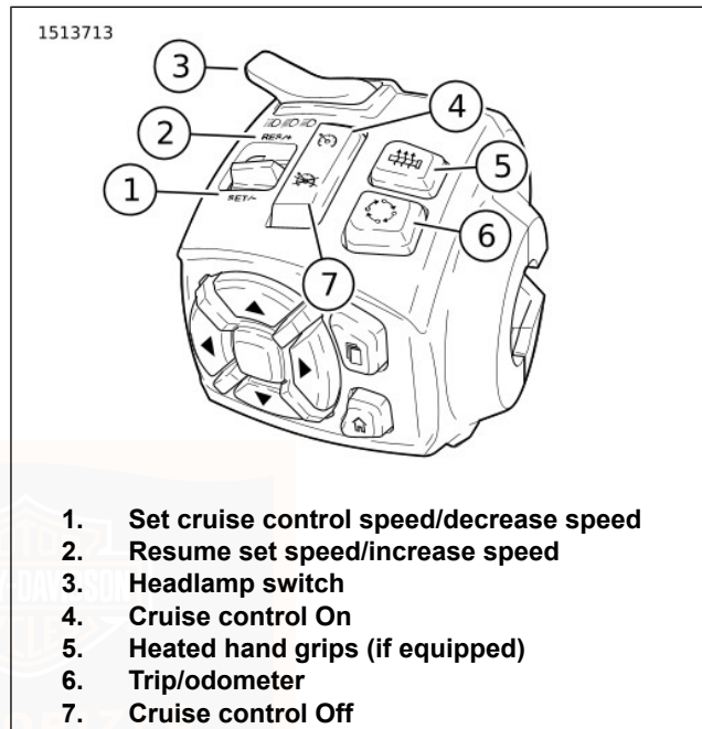
Figure 34. LHCM - Top
