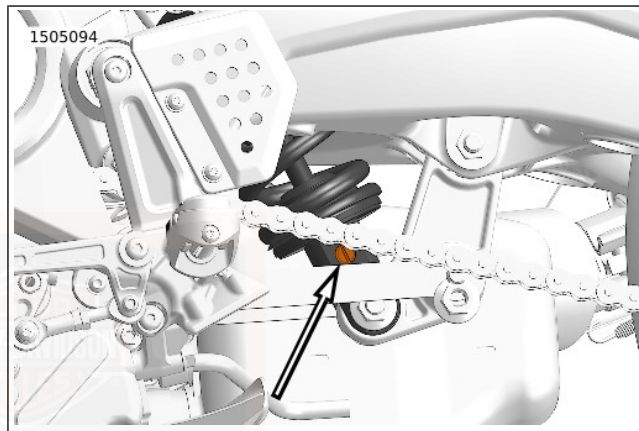
Figure 15. Rebound Adjuster
