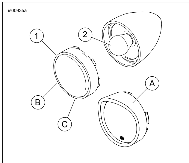
Figure 1. Service Parts: Bullet Style Turn Signal Trim Rings
