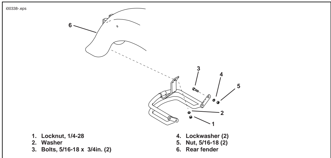
Illustration. Rear Fender Rail And Mounting Hardware
