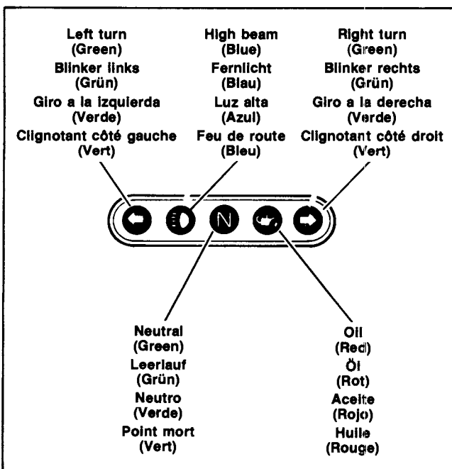
Figure 9. Indicator Lights
