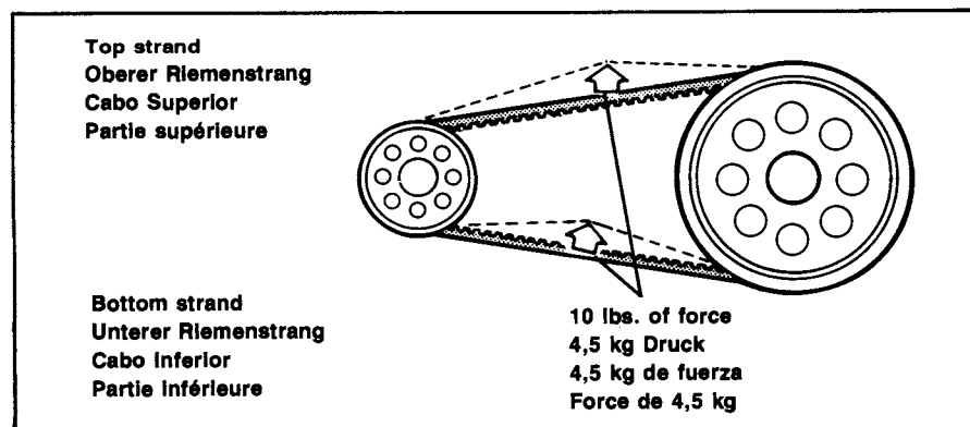
Figure 39. Belt Deflection
