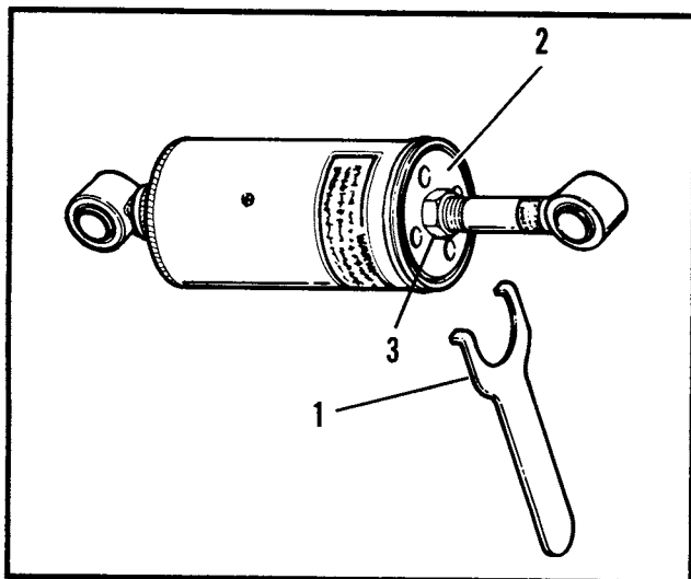
Figure 20. Shock Adjustment – Softail Models
