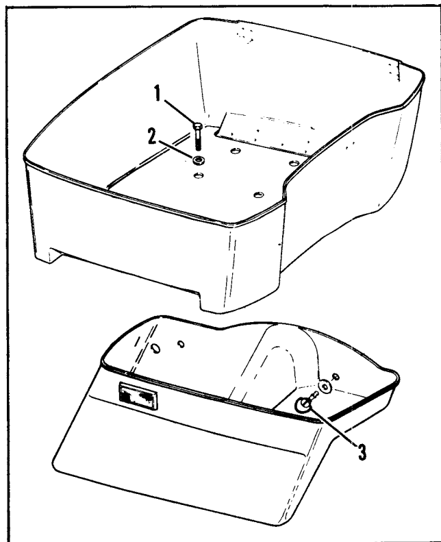
Figure 22. Tour-Pak and Saddlebag Installation - FLT
