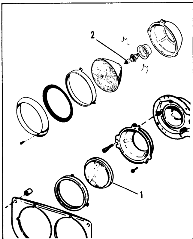
Figure 45. Headlamp
