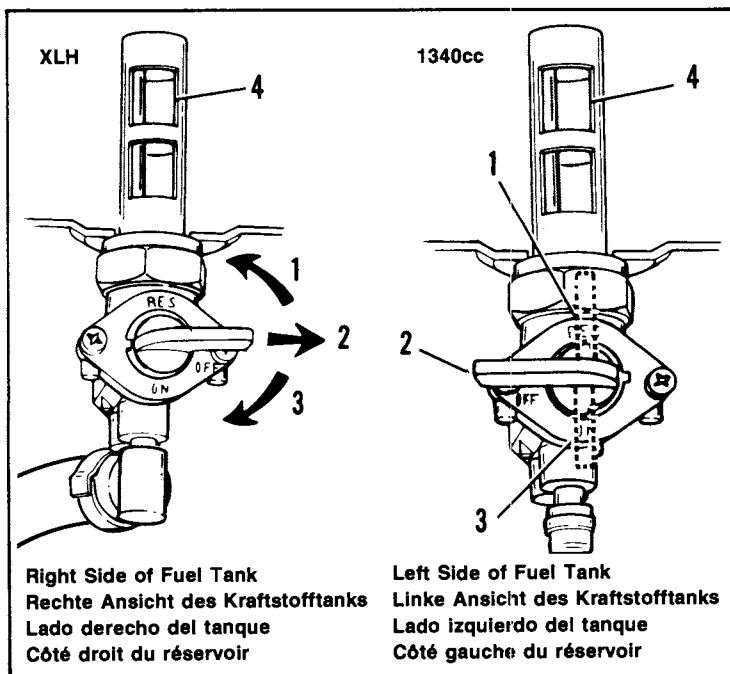
Figure 15. Fuel Supply Valve
