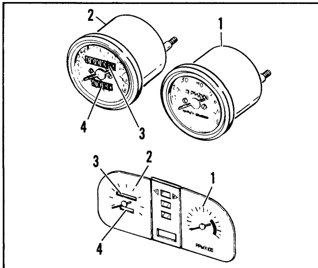
Figure 10. Speedometer, Odometer, Trip-Odometer, Tachometer
