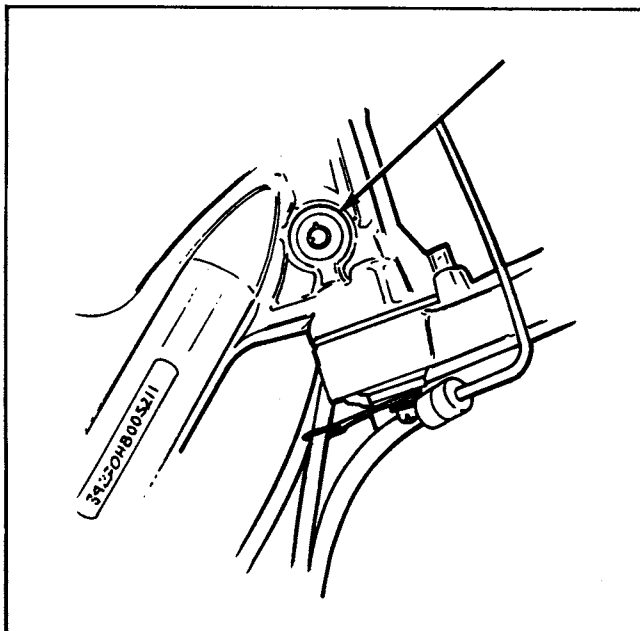
Figure 14. Dyna Glide Fork Lock
