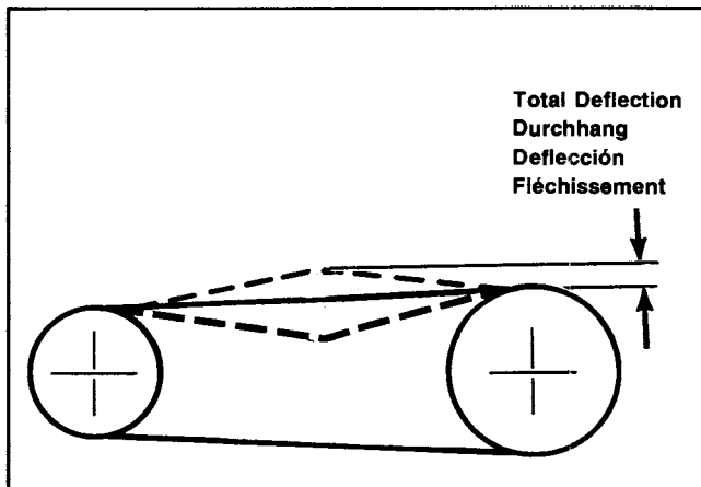
Figure 37. Primary Chain Free Play (Total Deflection)
