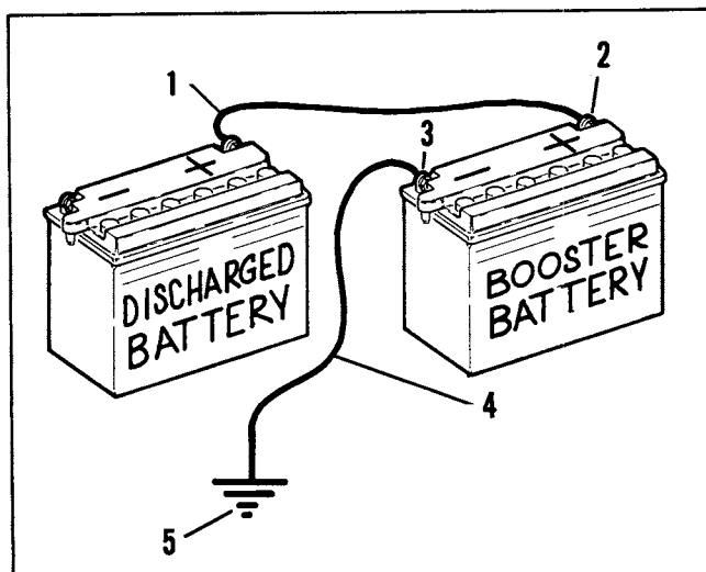
Figure 48. Jump Start Cable Connections
