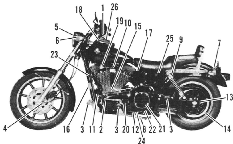
Dyna Glide – Left Side View (Typical)
