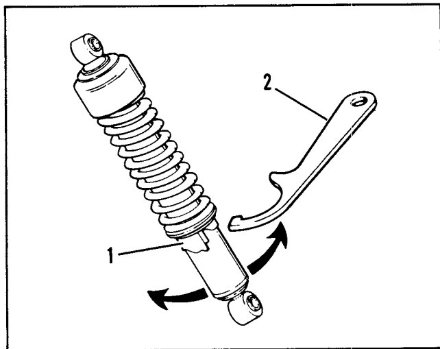
Figure 21. Shock Adjustment – FXR/S/SP/CON, FXD, XLH
