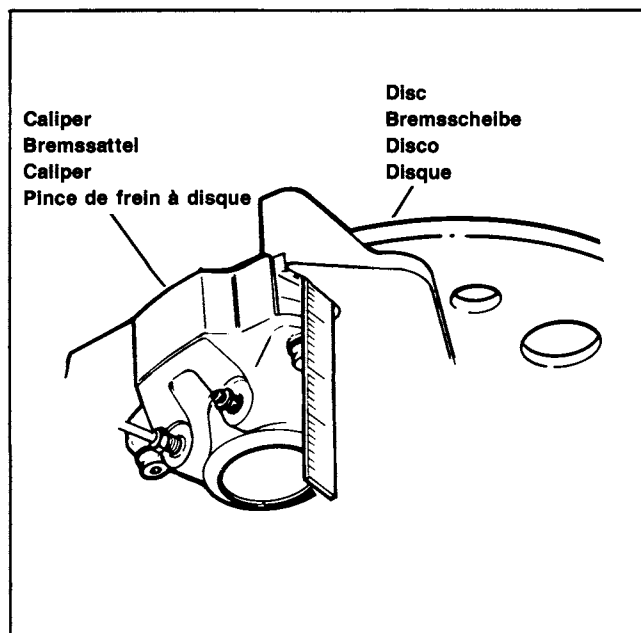
Figure 44. Measuring Rear Brake Outer Pad - XLH Models
