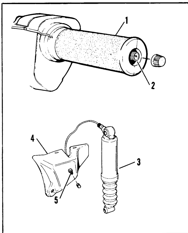
Figure 17. Air Suspension Components - FLT Models
