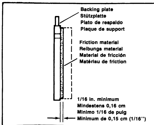
Figure 42. Brake Pad Side View
