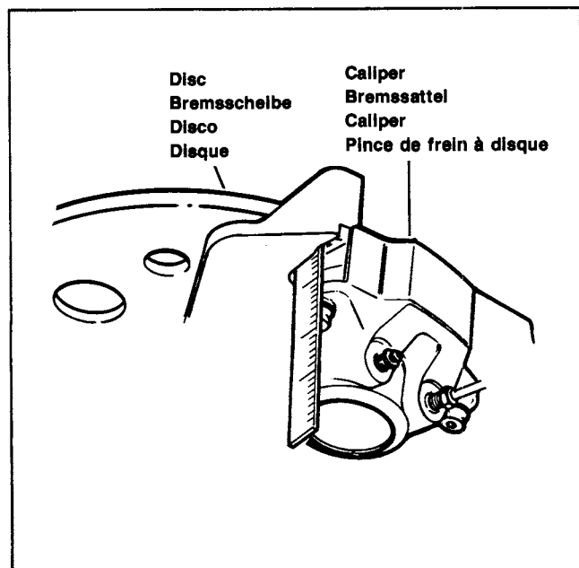
Figure 43. Measuring Rear Brake Outer Pad - 1340cc Models (Typical)
