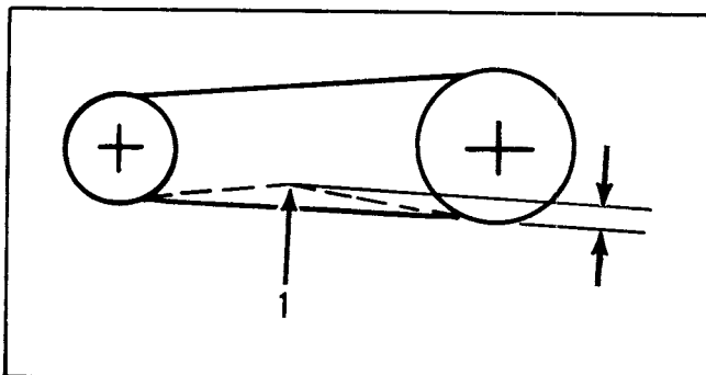
Figure 38. XLH 883 Rear Chain Deflection
