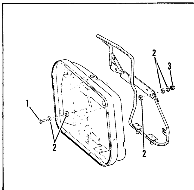
Figure 24. Saddlebag Installation - FXRT
