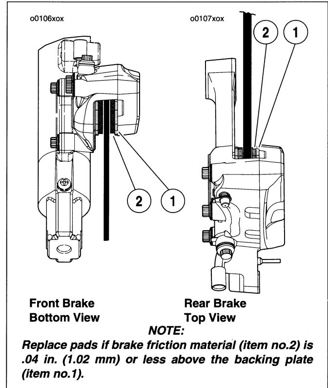
Figure 42. Brake Pads
