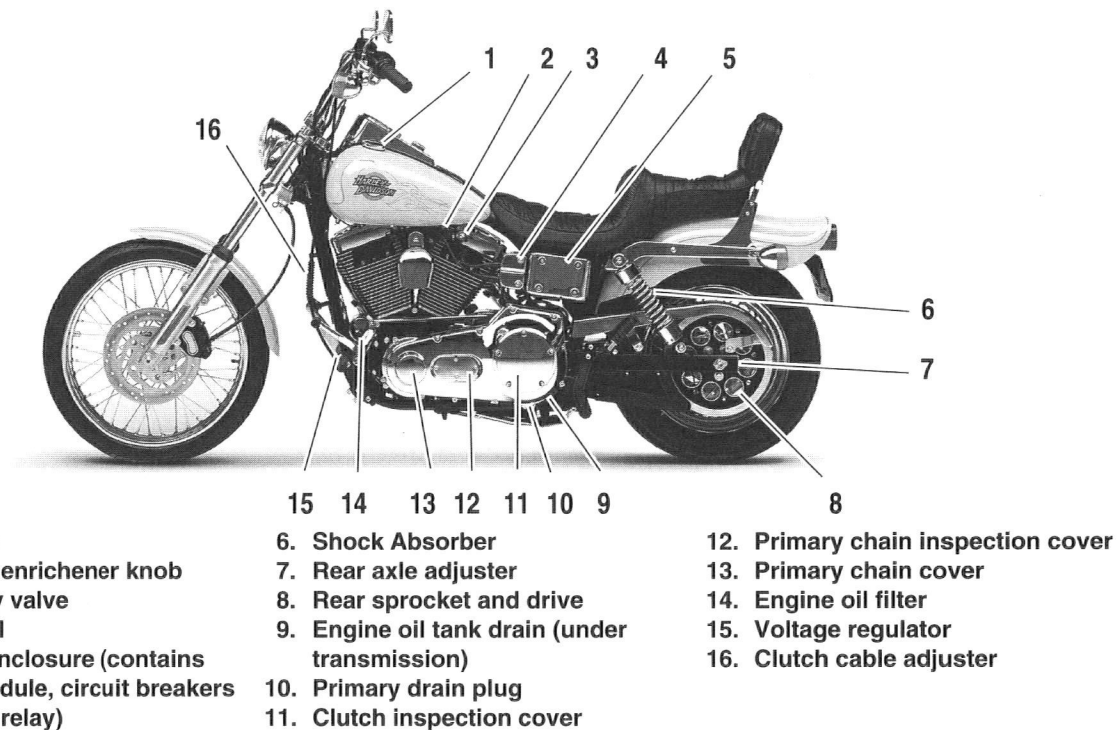
Figure 4. Dyna Wide Glide (FXDWG) - Left Side View
