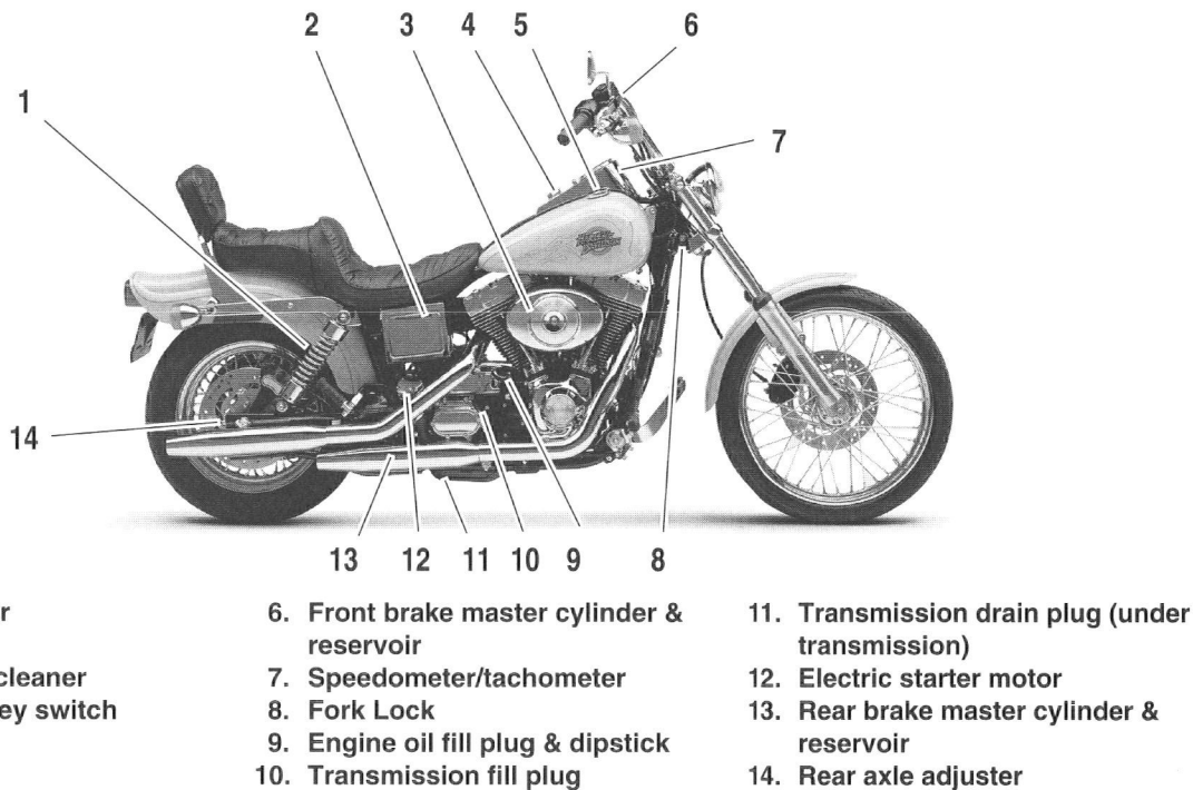
Figure 5. Dyna Wide Glide (FXDWG) - Right Side View
