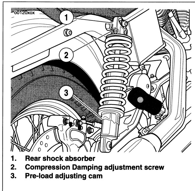
Figure 23. Dyna Rear Shock Absorber
