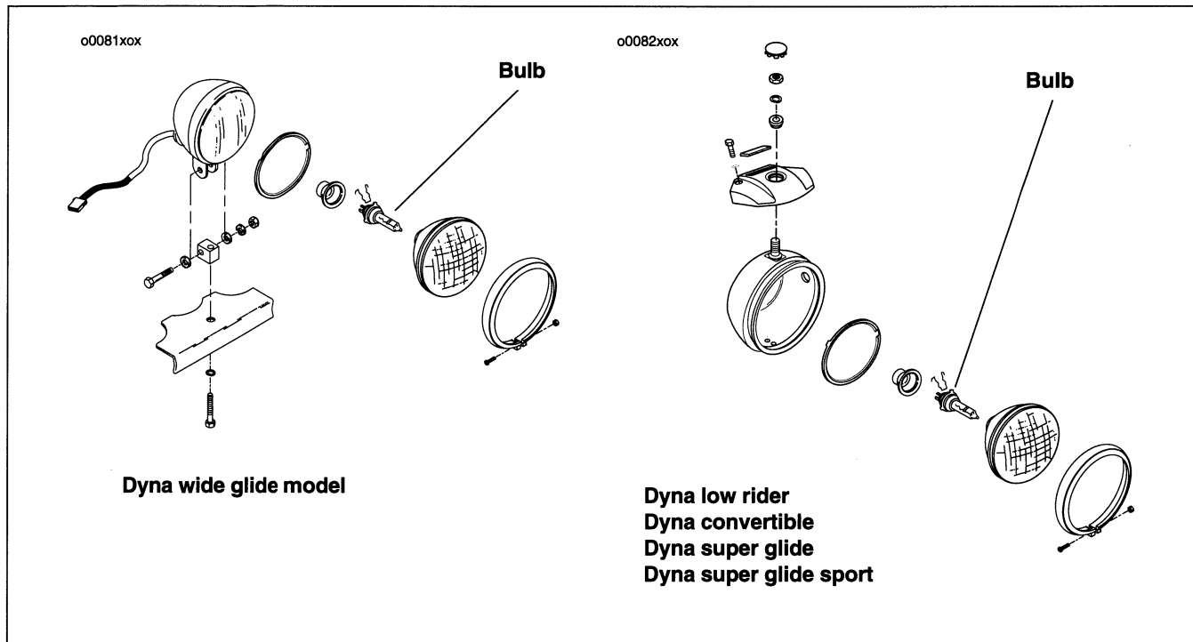
Figure 43. Dyna Headlamps
