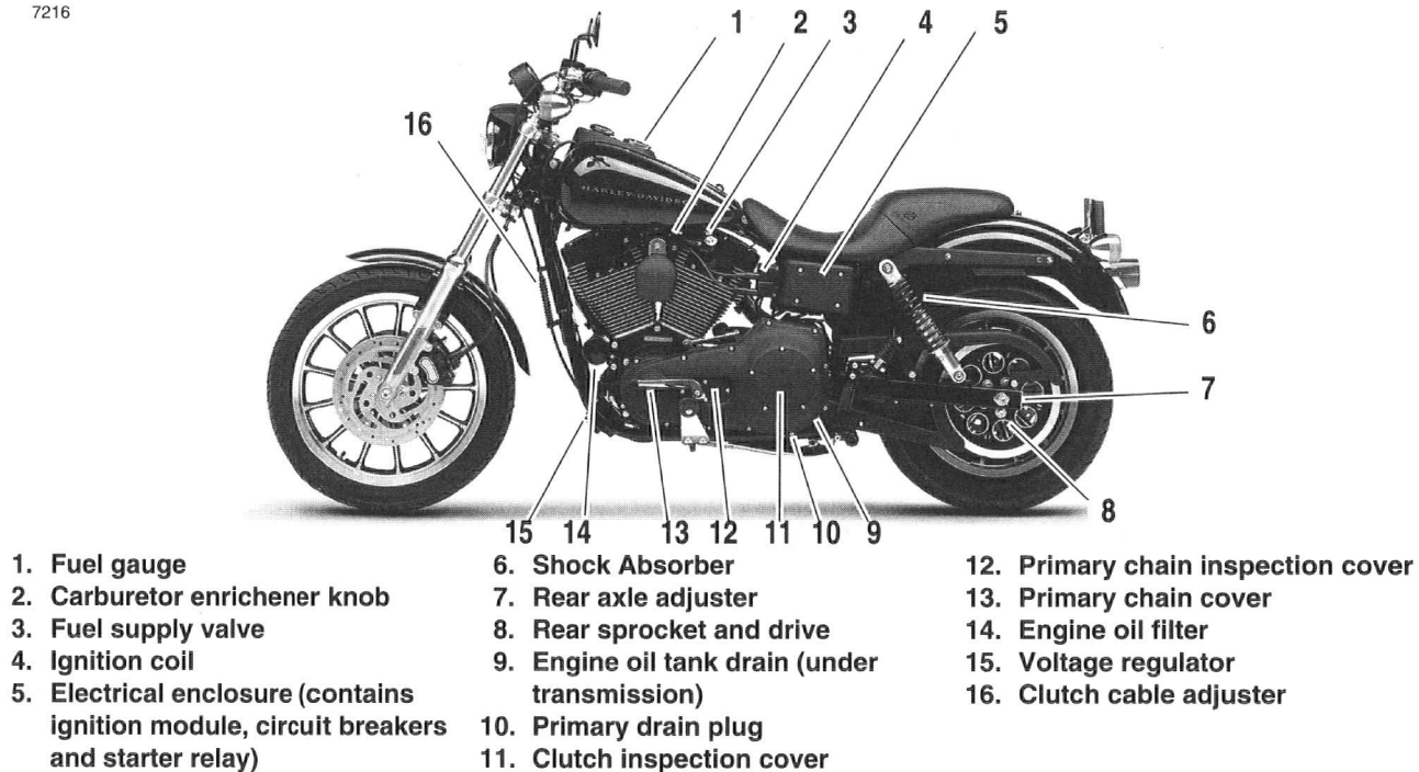
Figure 10. Dyna Super Glide Sport (FXDX) - Left Side View
