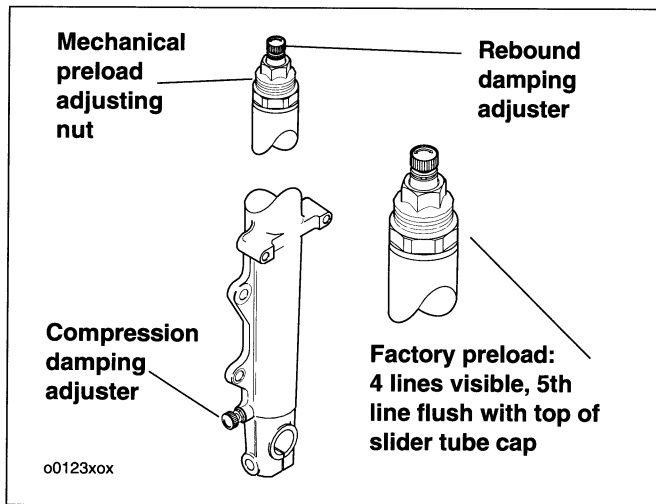
Figure 26. Front Suspension Adjustments
