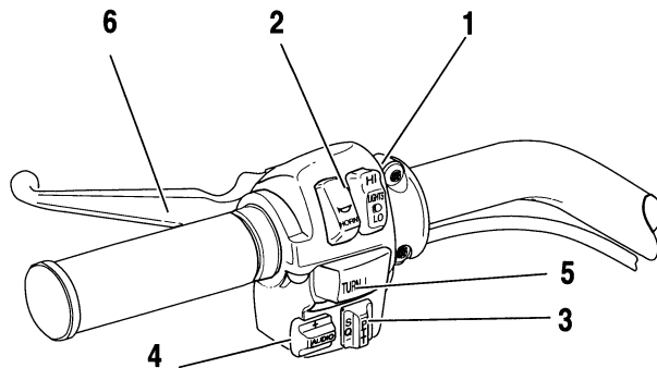
Figure 12. Hand Controls (Typical)
