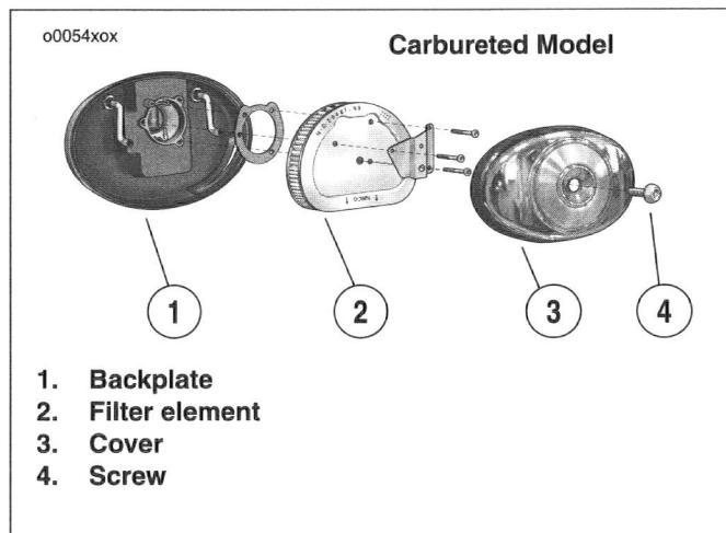
Figure 41. Air Cleaner
