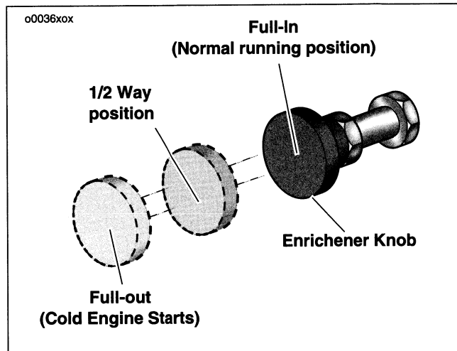
Figure 13. Setting the Enrichener
