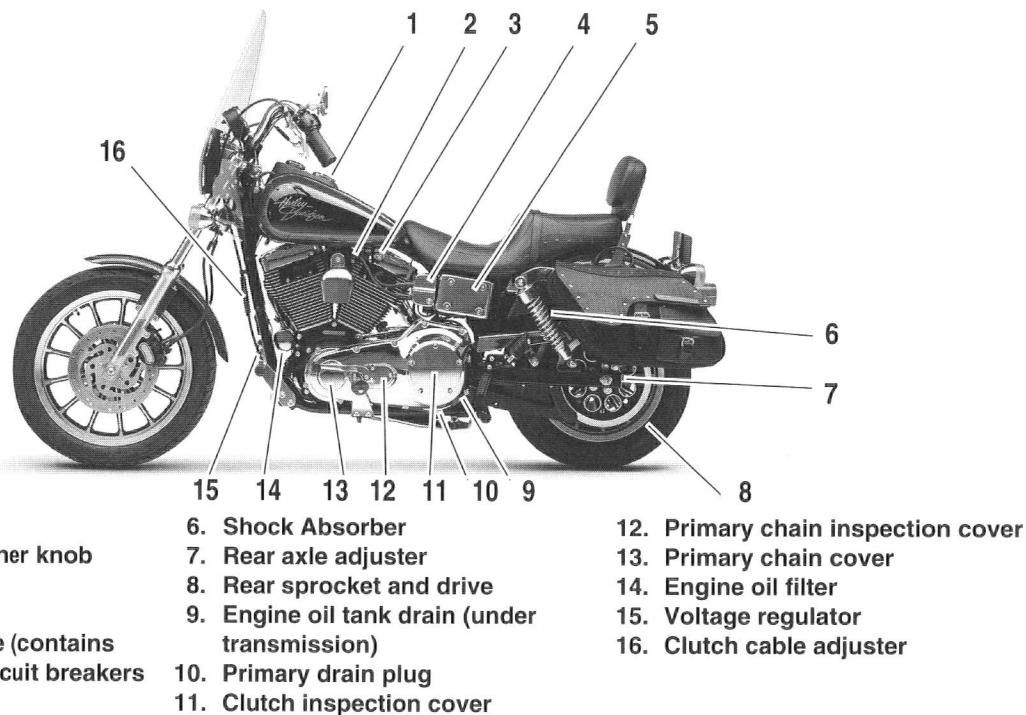
Figure 6. Dyna Glide Convertible (FXDX-CONV) - Left Side View
