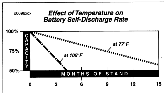
Figure 35. Battery Self-Discharging Rate
