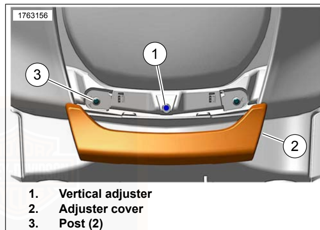
Figure 116. Headlamp Adjustment
