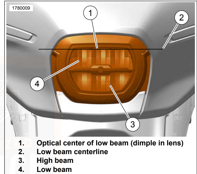
Figure 112. Headlamp Components
