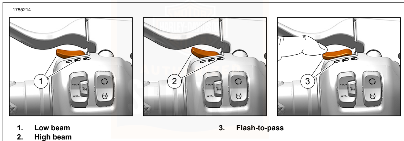
Figure 28. Headlamp Switch
