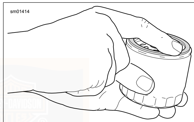
Figure 86. Lubricating New Oil Filter Gasket LOW TEMPERATURE LUBRICATION
