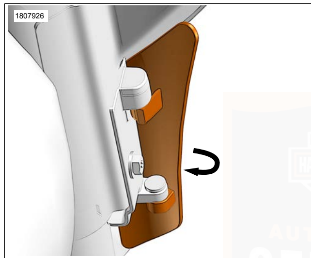
Figure 59. Air Deflector: Fork Mounted Fairing
