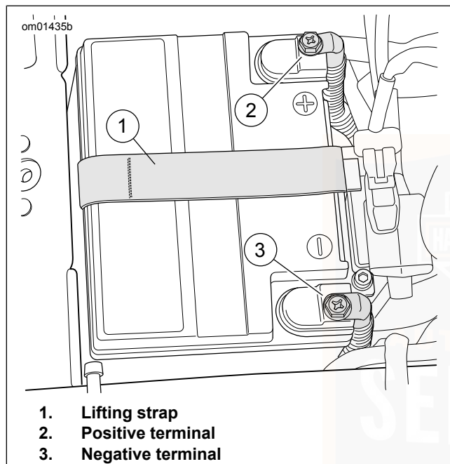
Figure 109. Battery Compartment
