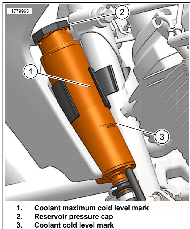
Figure 96. Coolant Level
