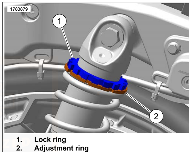
Figure 13. Threaded Adjuster (Right Side Shock Absorber)
