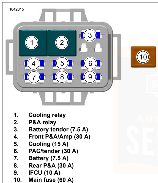
Figure 111. Fuses and Relays Identification
