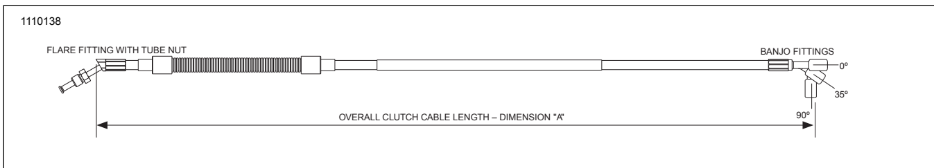
Figure 3-3. Hydraulic Clutch Lines
