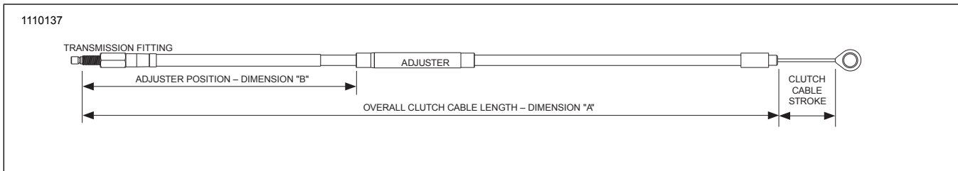
Figure 3-2. Clutch Cables
