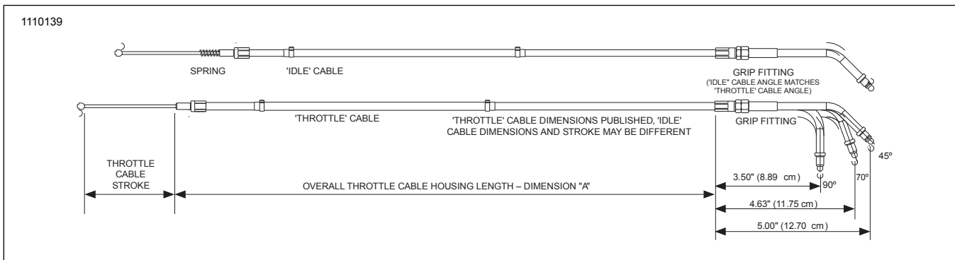
Figure 3-4. Throttle/Idle Cables
