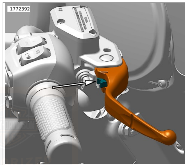
Figure 27. Front Brake Lever Adjustment Thumbwheel
