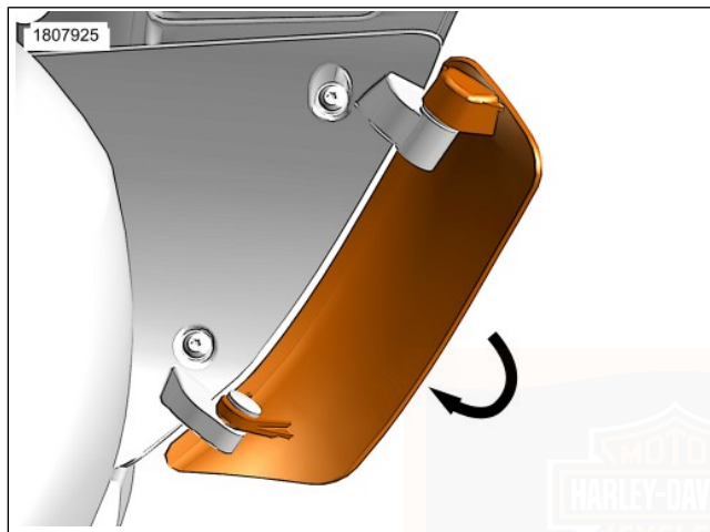
Figure 59. Air Deflector
