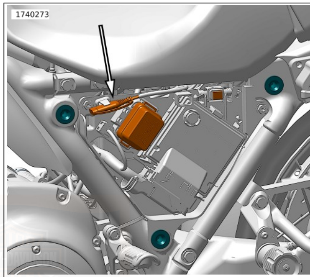
Figure 105. Battery Tender Connector (under left side cover)
