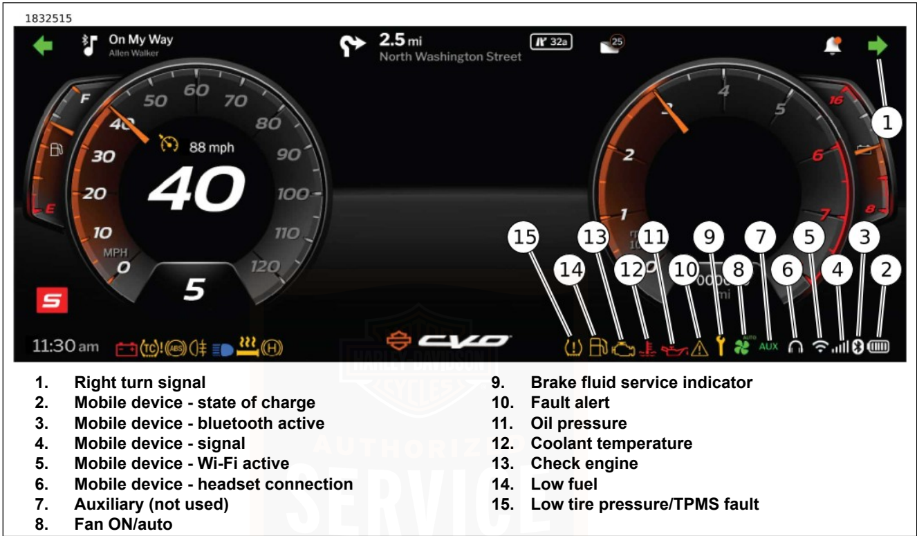
Figure 30. ICU Indicators
