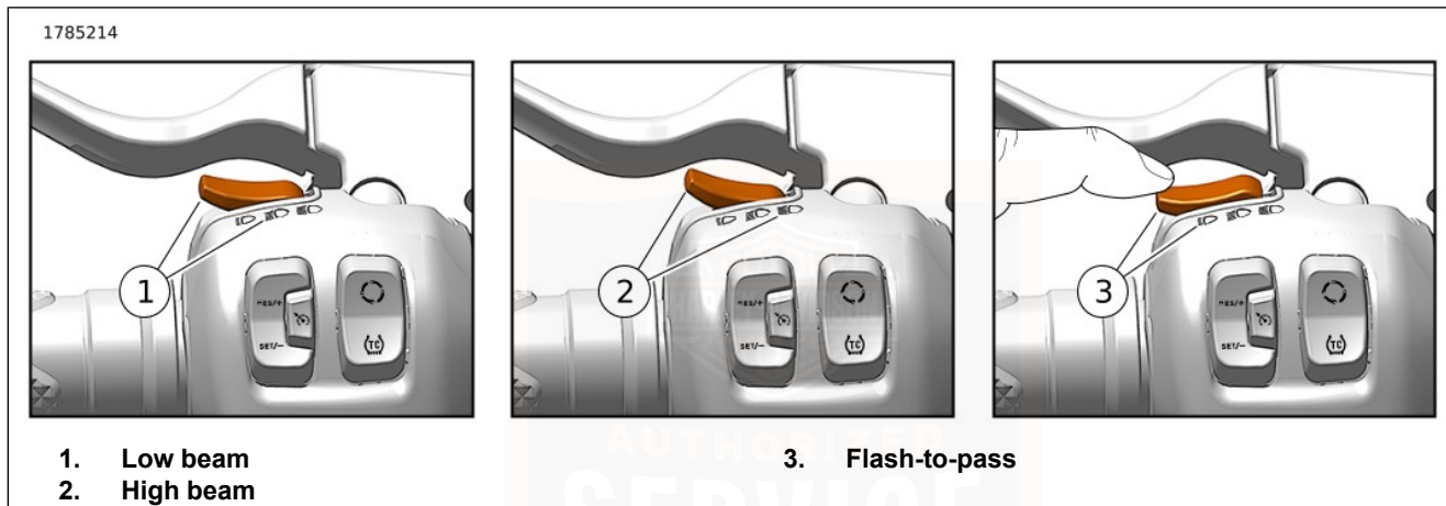
Figure 31. Headlamp Switch
