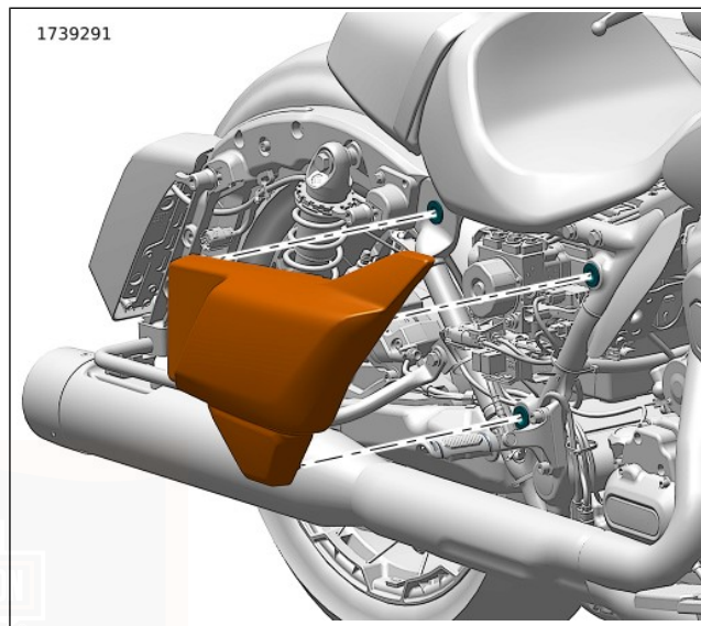
Figure 104. Side Cover
