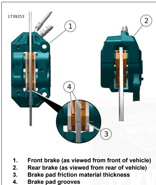
Figure 96. Brake Pad Friction Material
