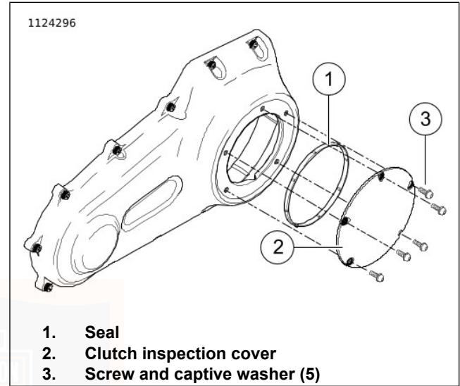
Figure 93. Clutch Cover (Typical)
