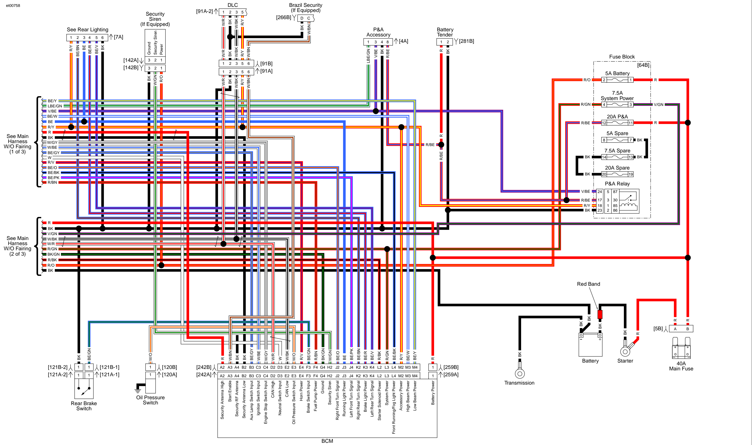
Main Harness (3 of 3): 2016 Touring (without Fairing)
