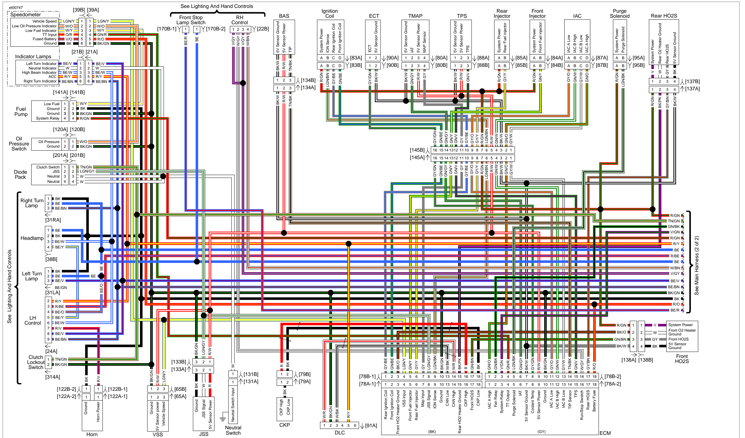
Main Harness (1 of 2): 2016 Street
