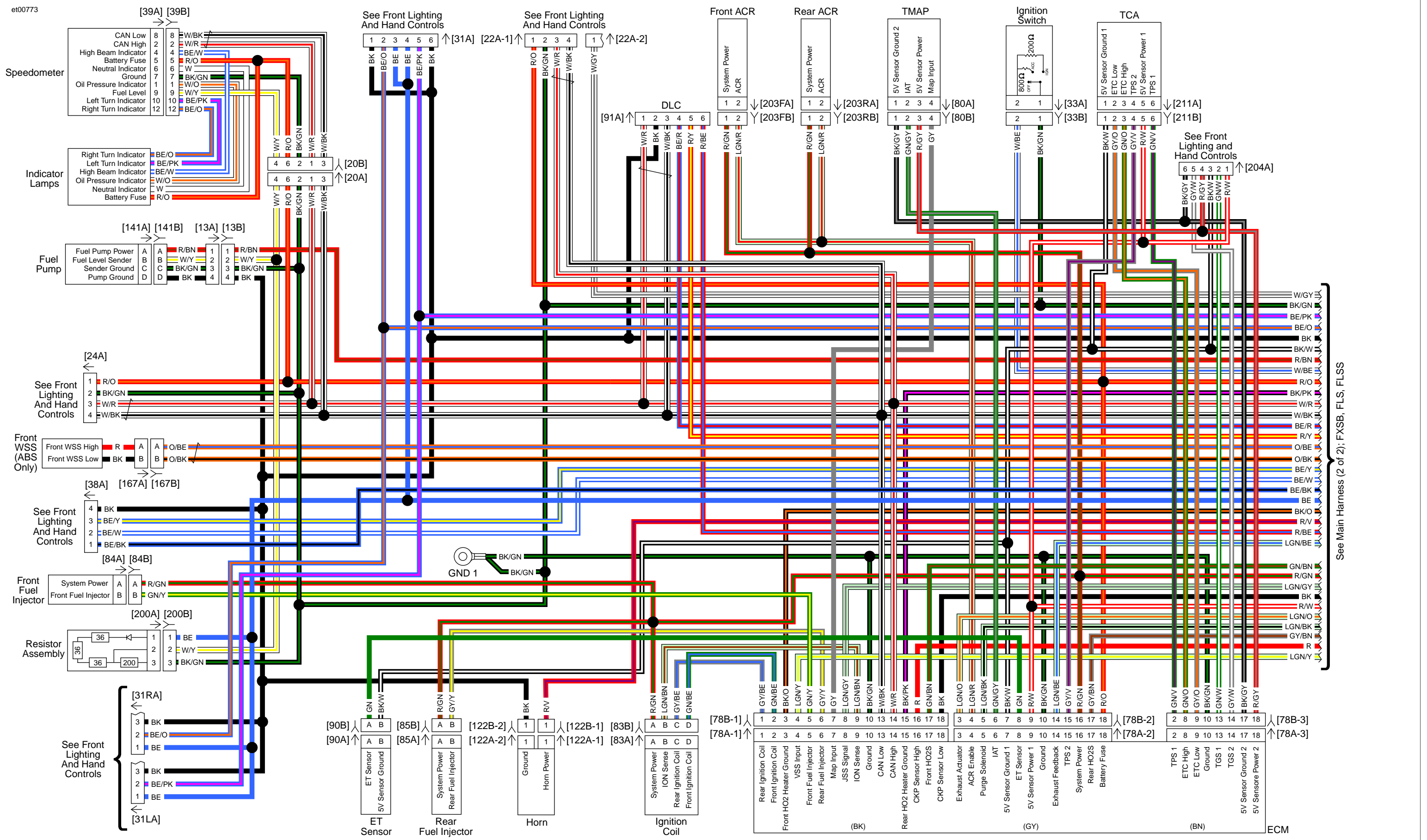
Main Harness 1 of 2: 2016 Softail (FLS, FLSS)
