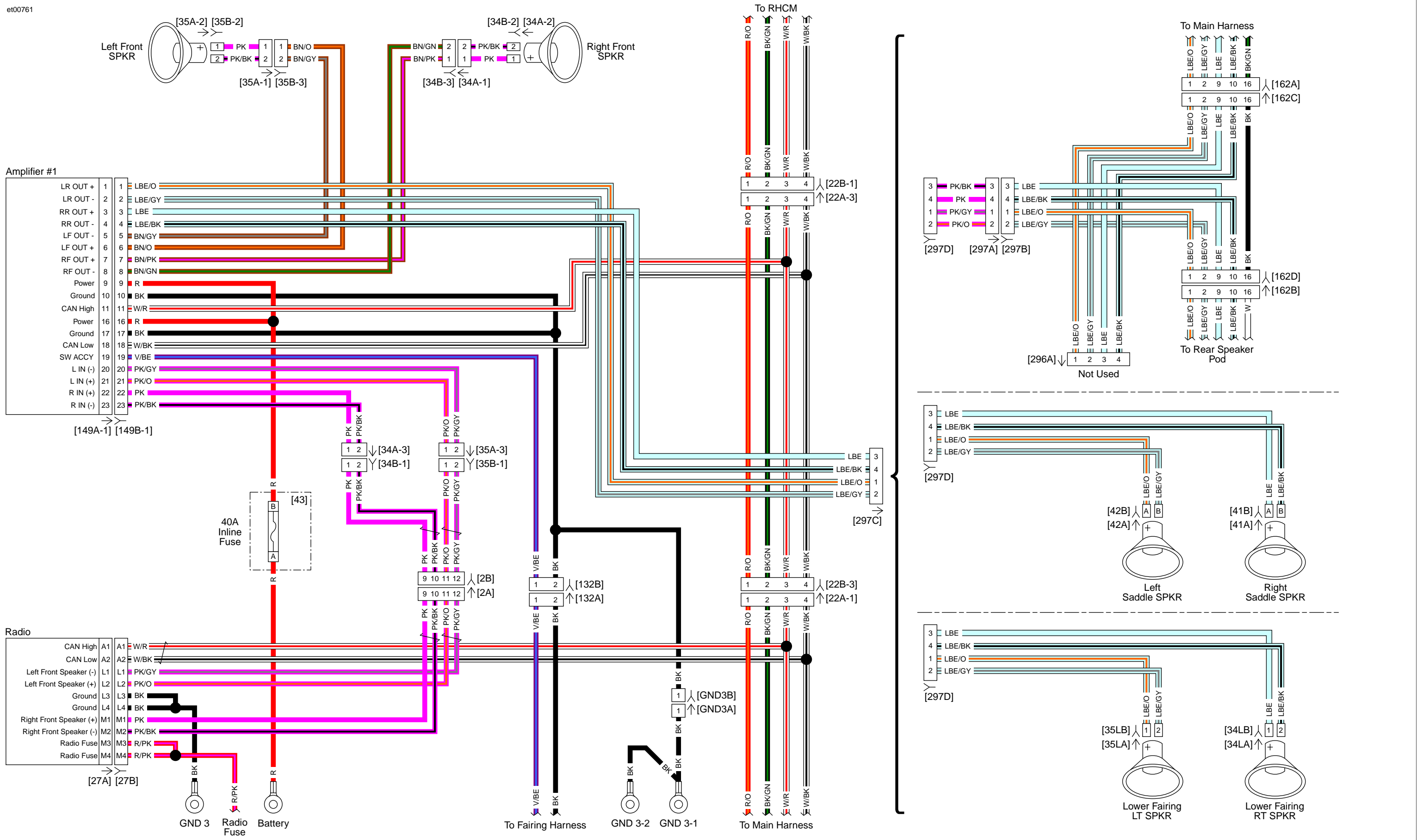
P&A Radio with 1 Amp: 2016 Touring
