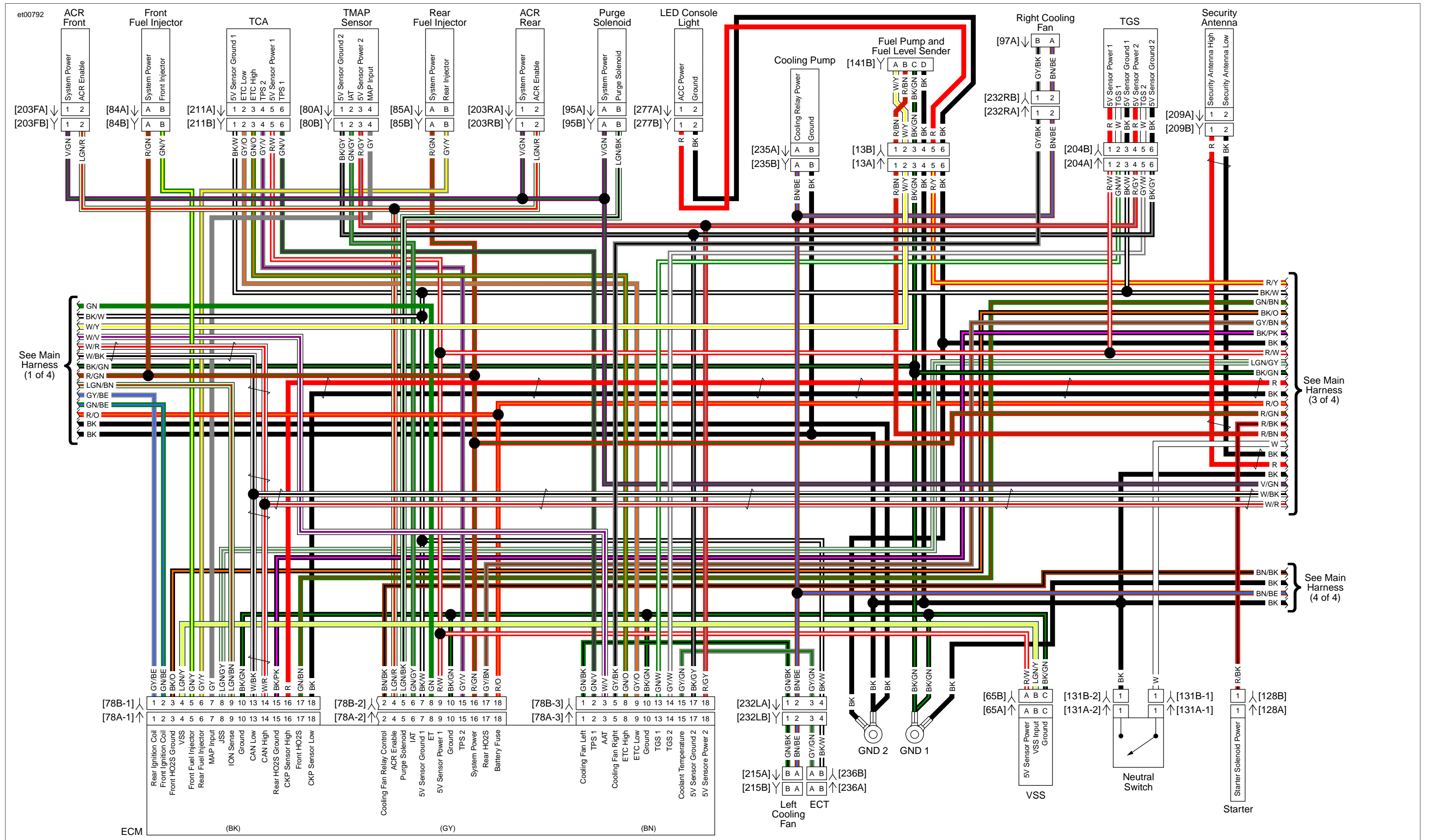
Main Harness (2 of 4): 2016 FLHXSE
