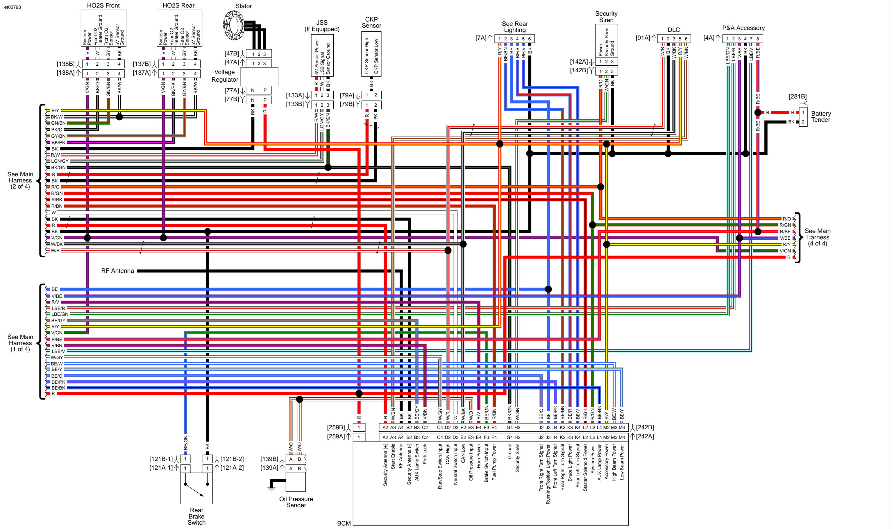
Main Harness (3 of 4): 2016 FLHXSE
