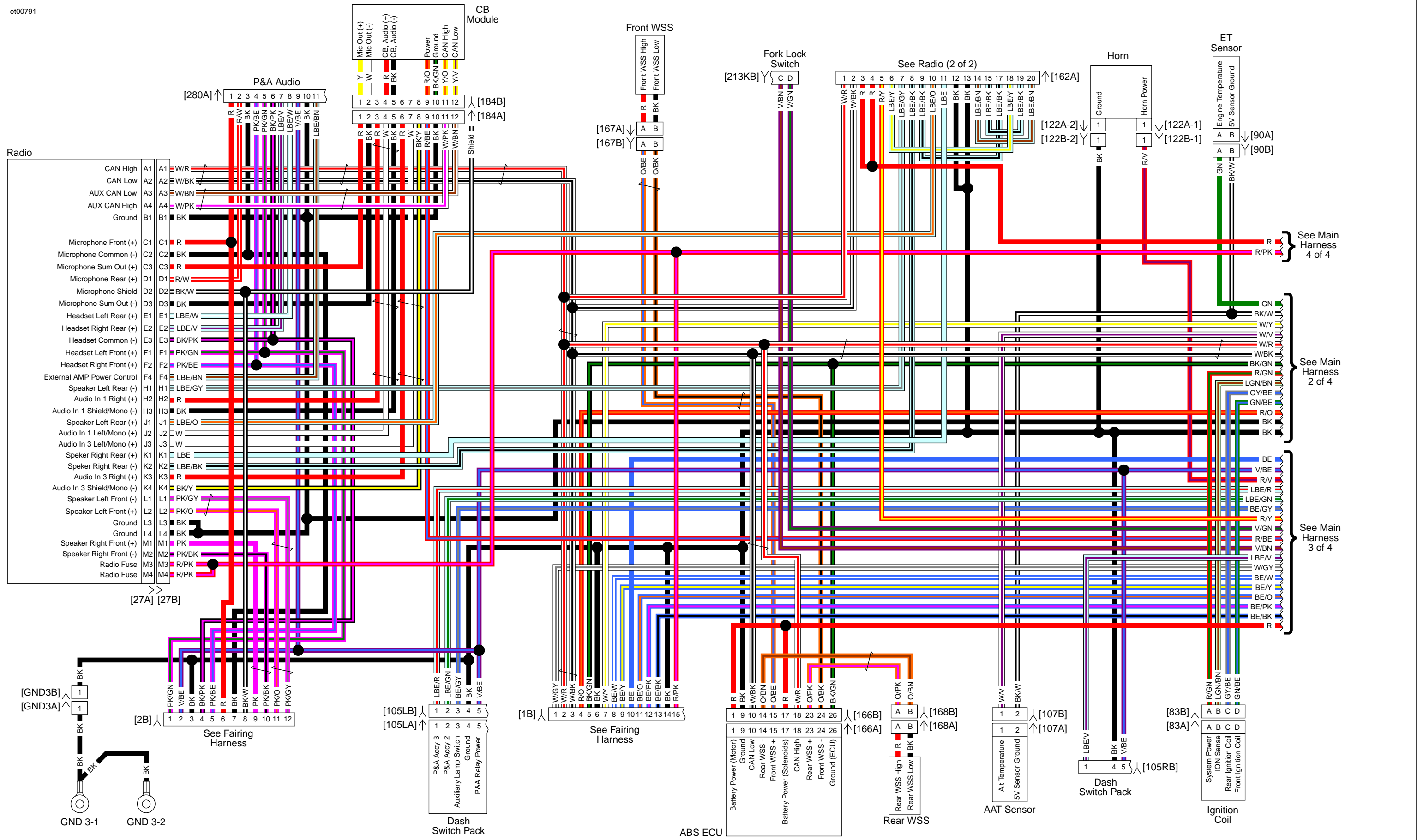
Main Harness (1 of 4): 2016 FLHXSE
