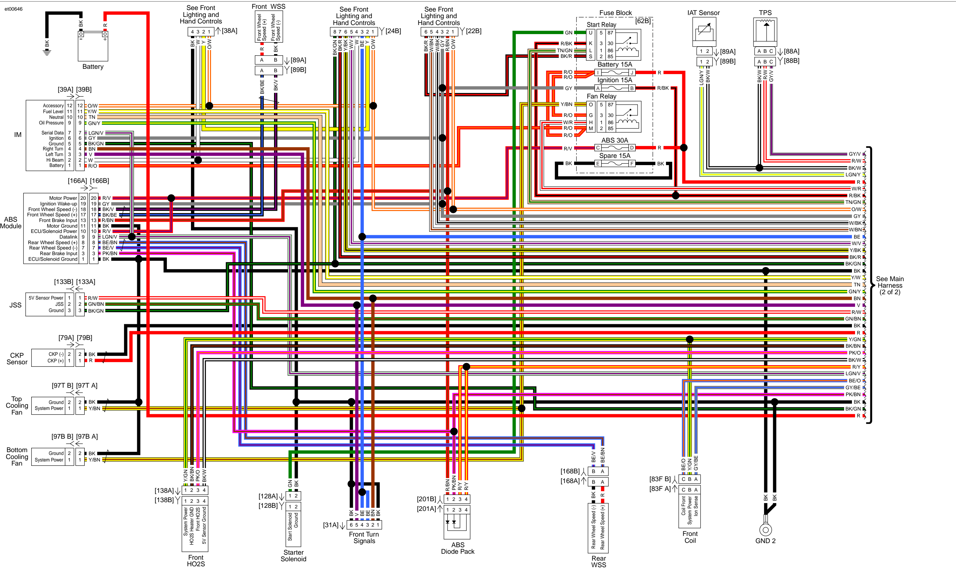
Main Harness (1 of 2): 2016 V-Rod
