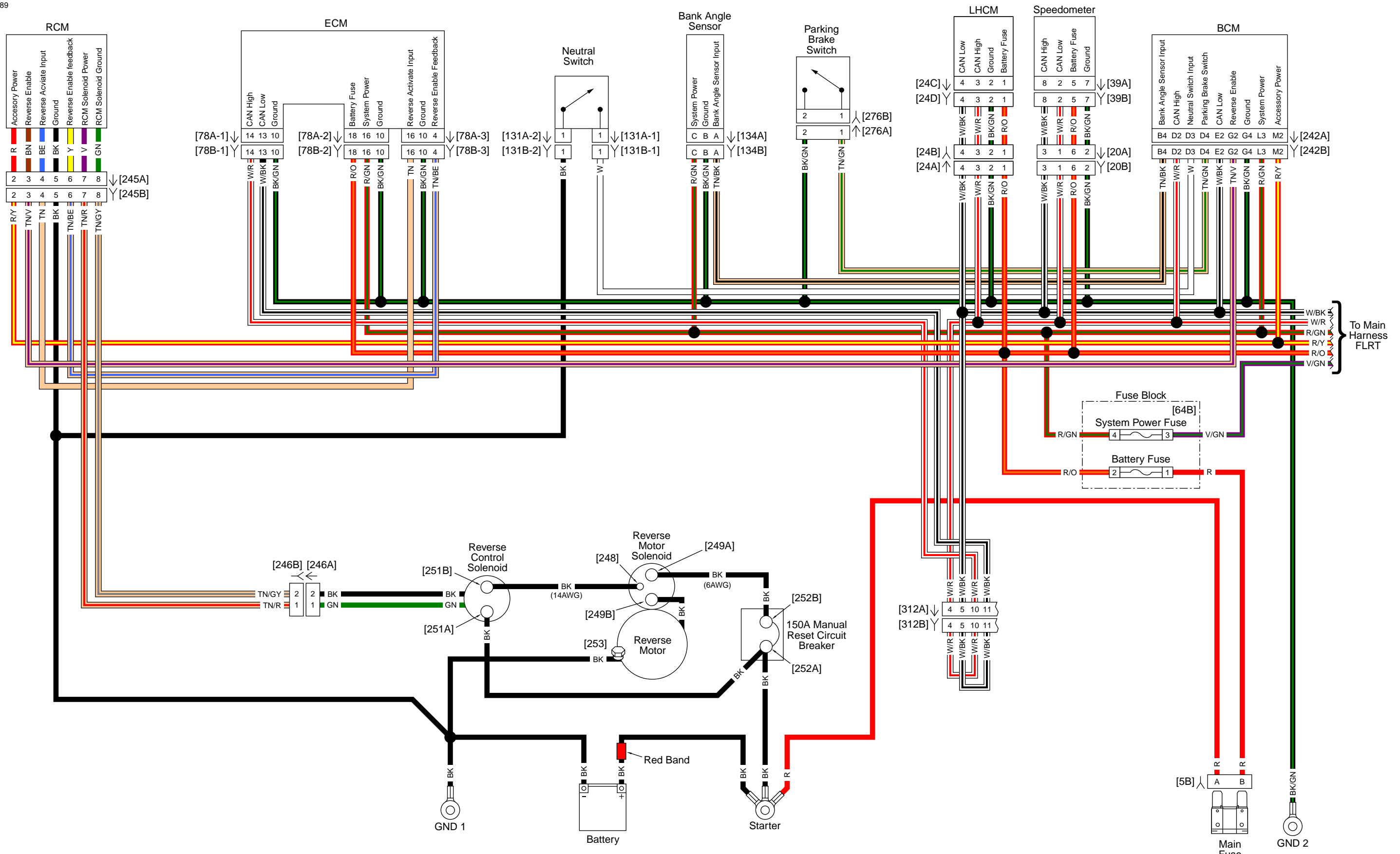
Reverse FLRT: 2016 Trike Model
