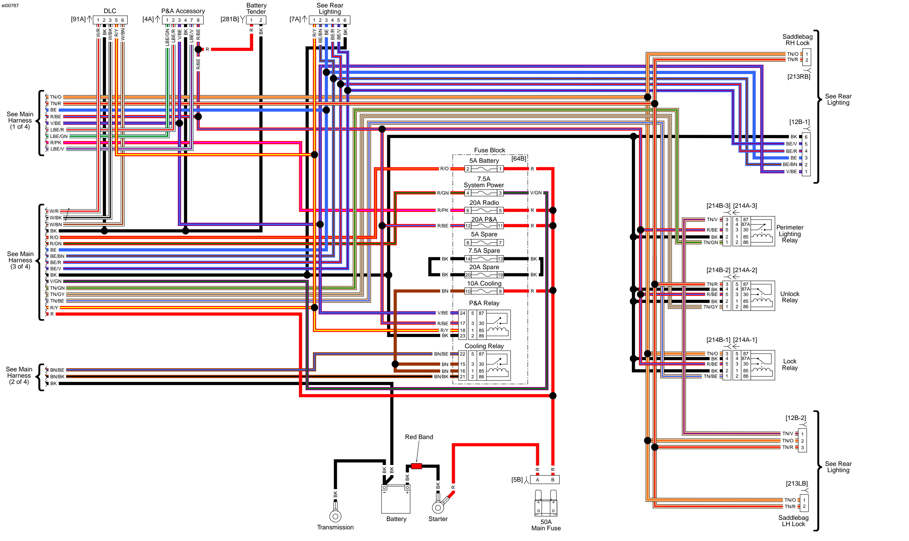
Main Harness (4 of 4): 2016 FLTRUSE
