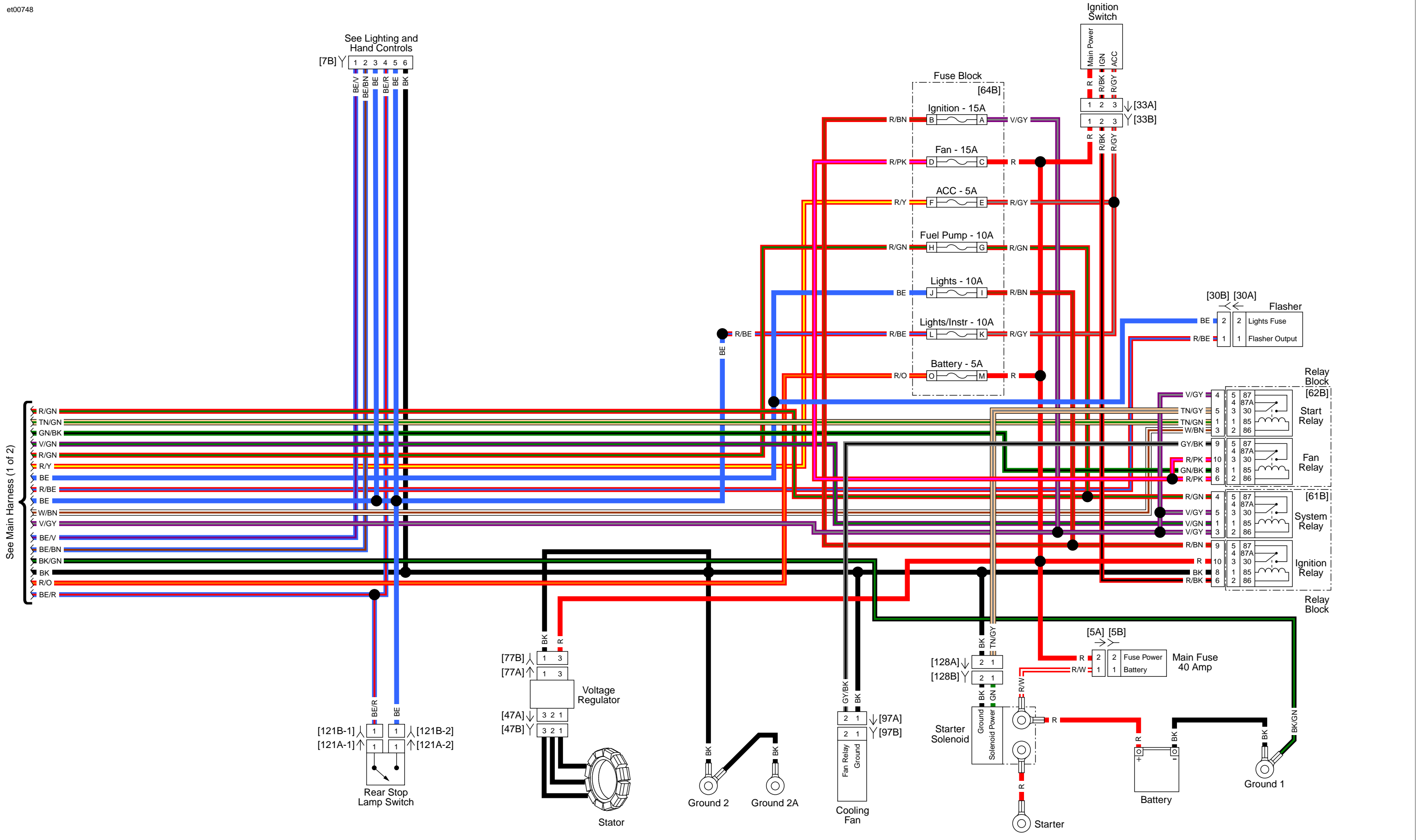
Main Harness (2 of 2): 2016 Street
