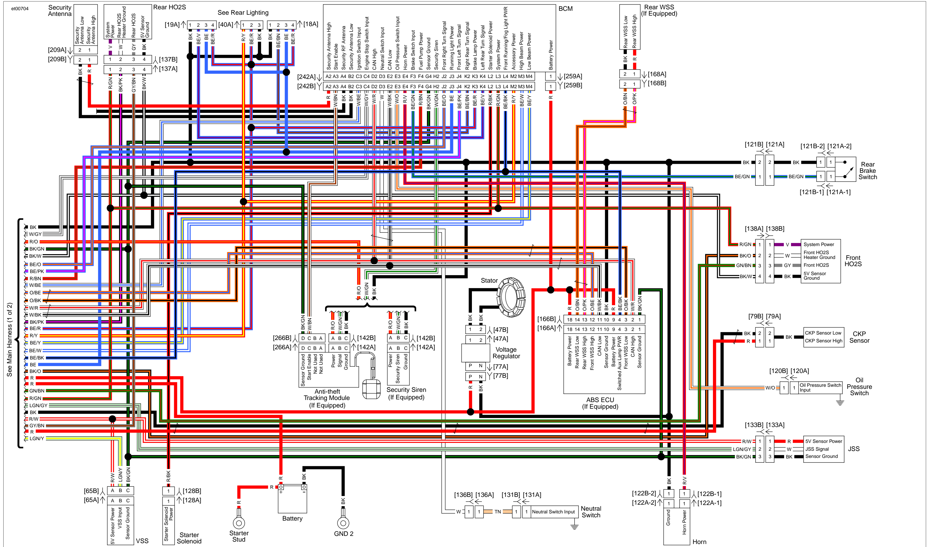
Main Harness 2 of 2: 2016 Sportster
