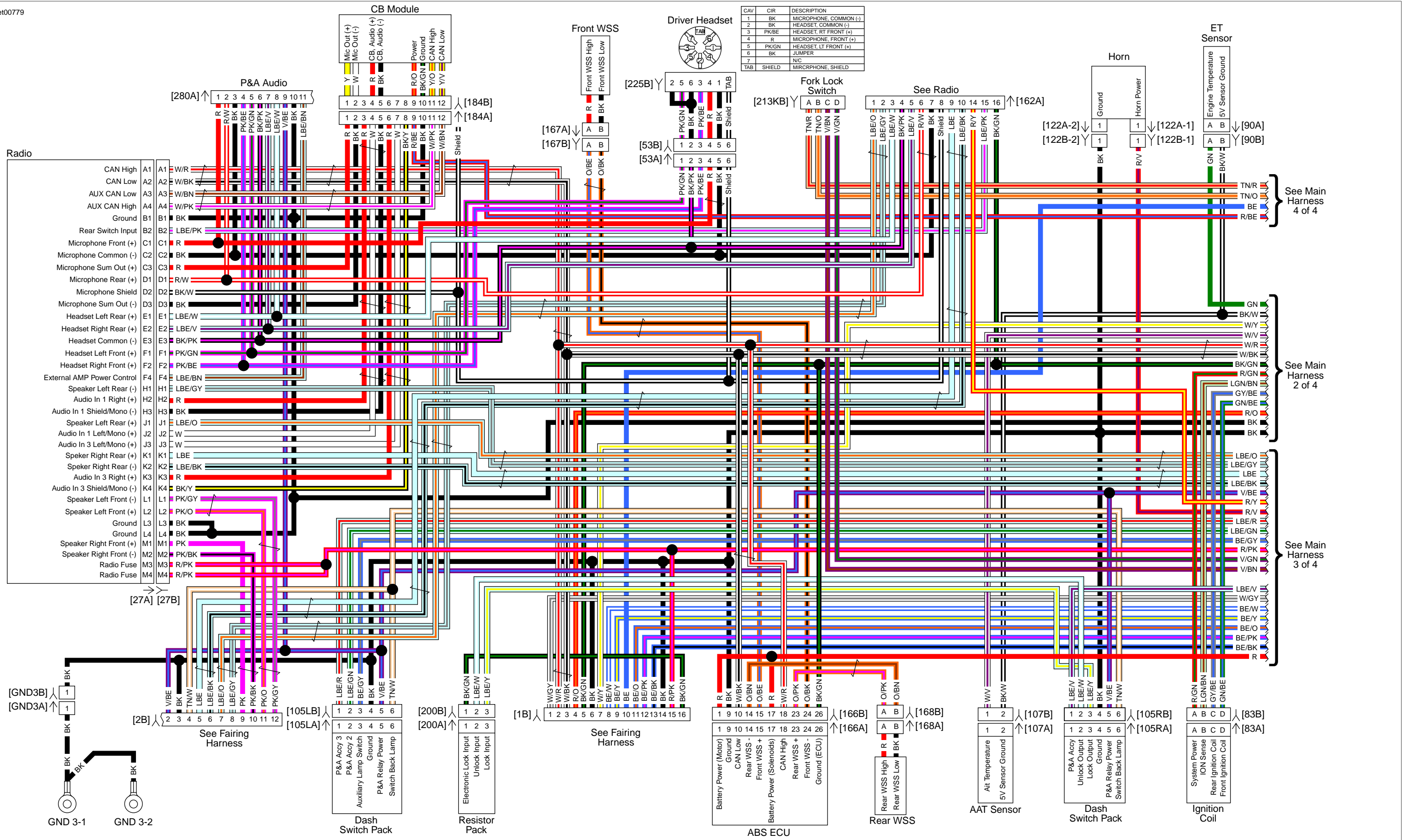
Main Harness (1 of 4): 2016 FLHTKSE
