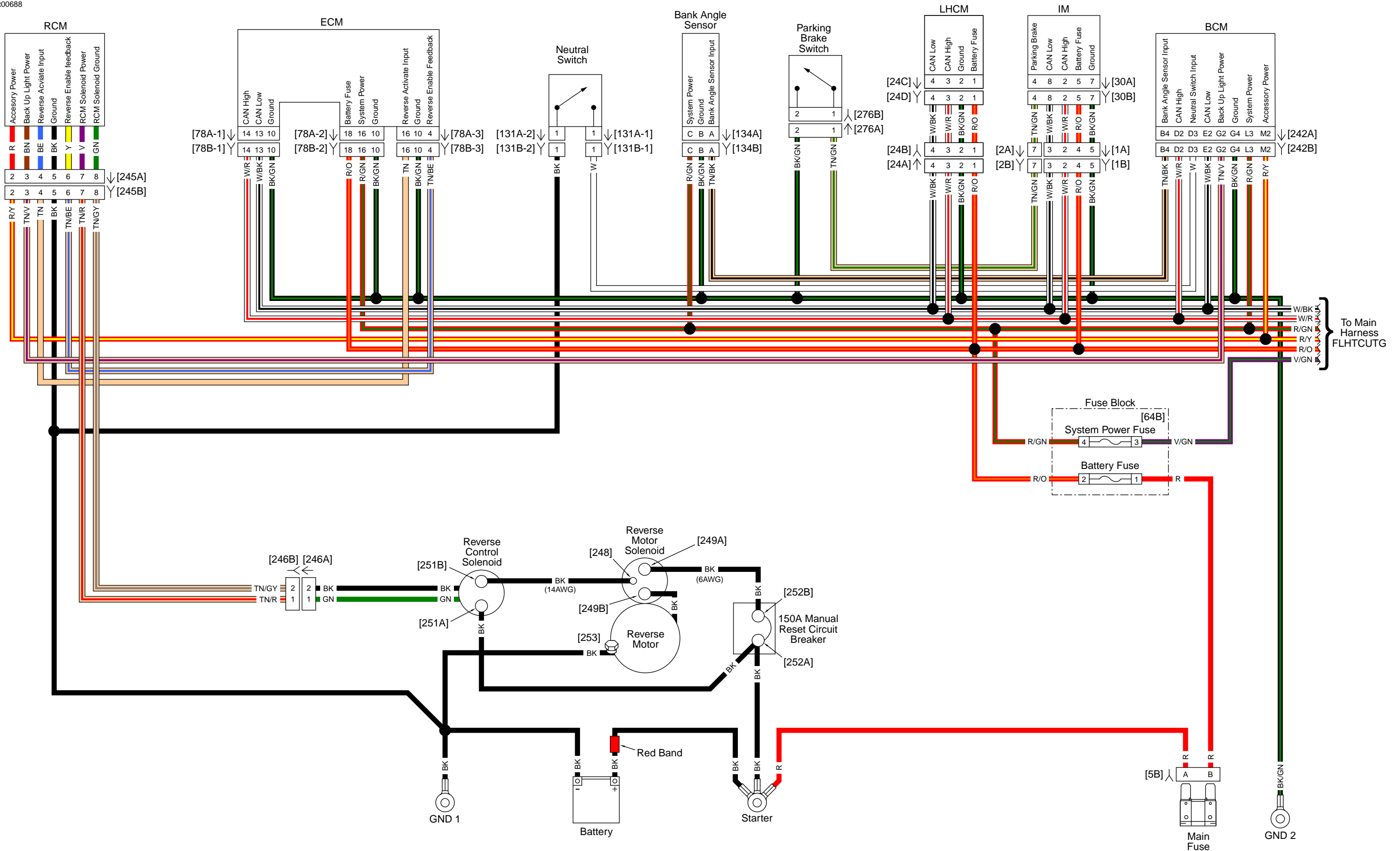
Reverse FLHTCUTG: 2016 Trike Model
