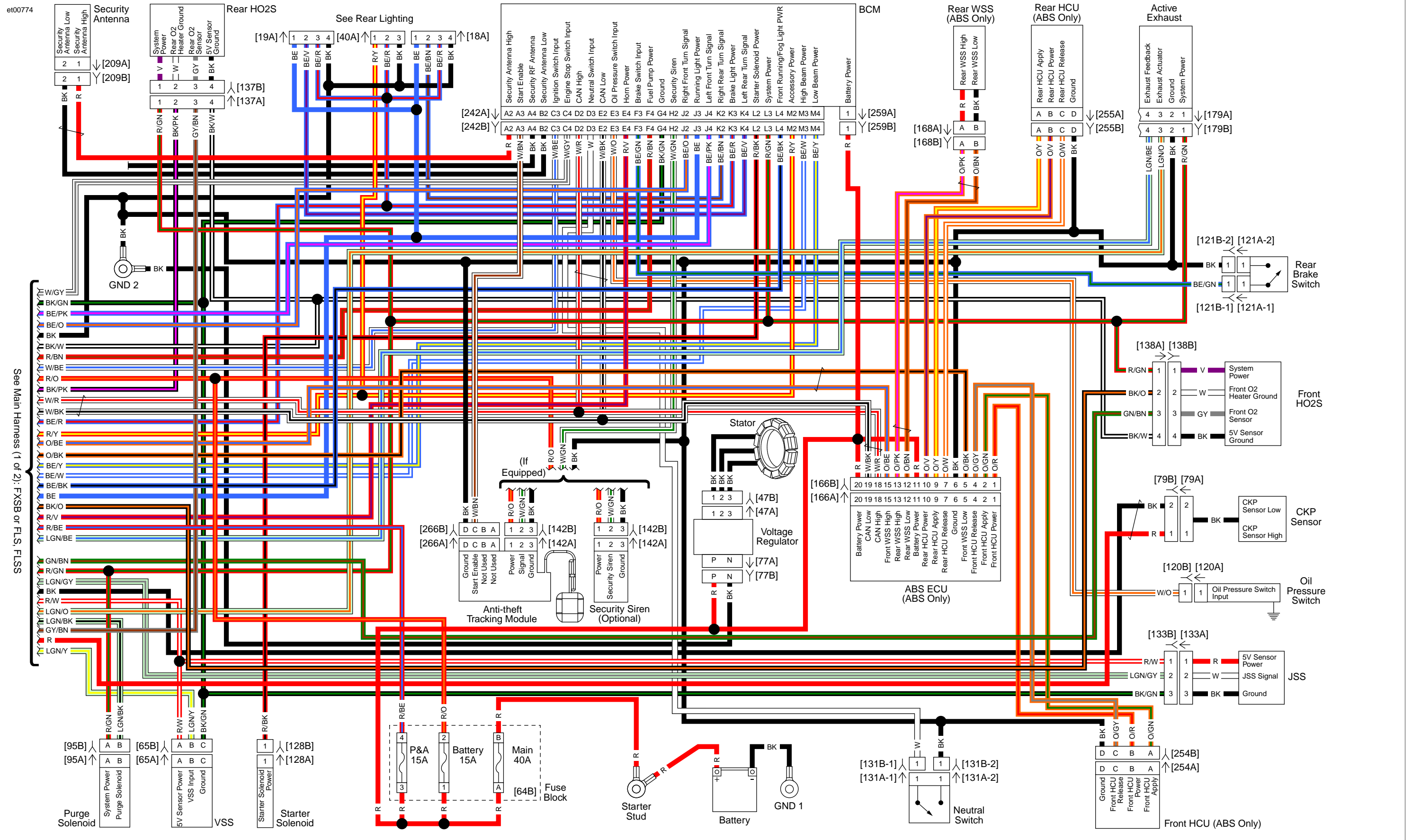
Main Harness 2 of 2: 2016 Softail (FXSB, FLS, FLSS)
