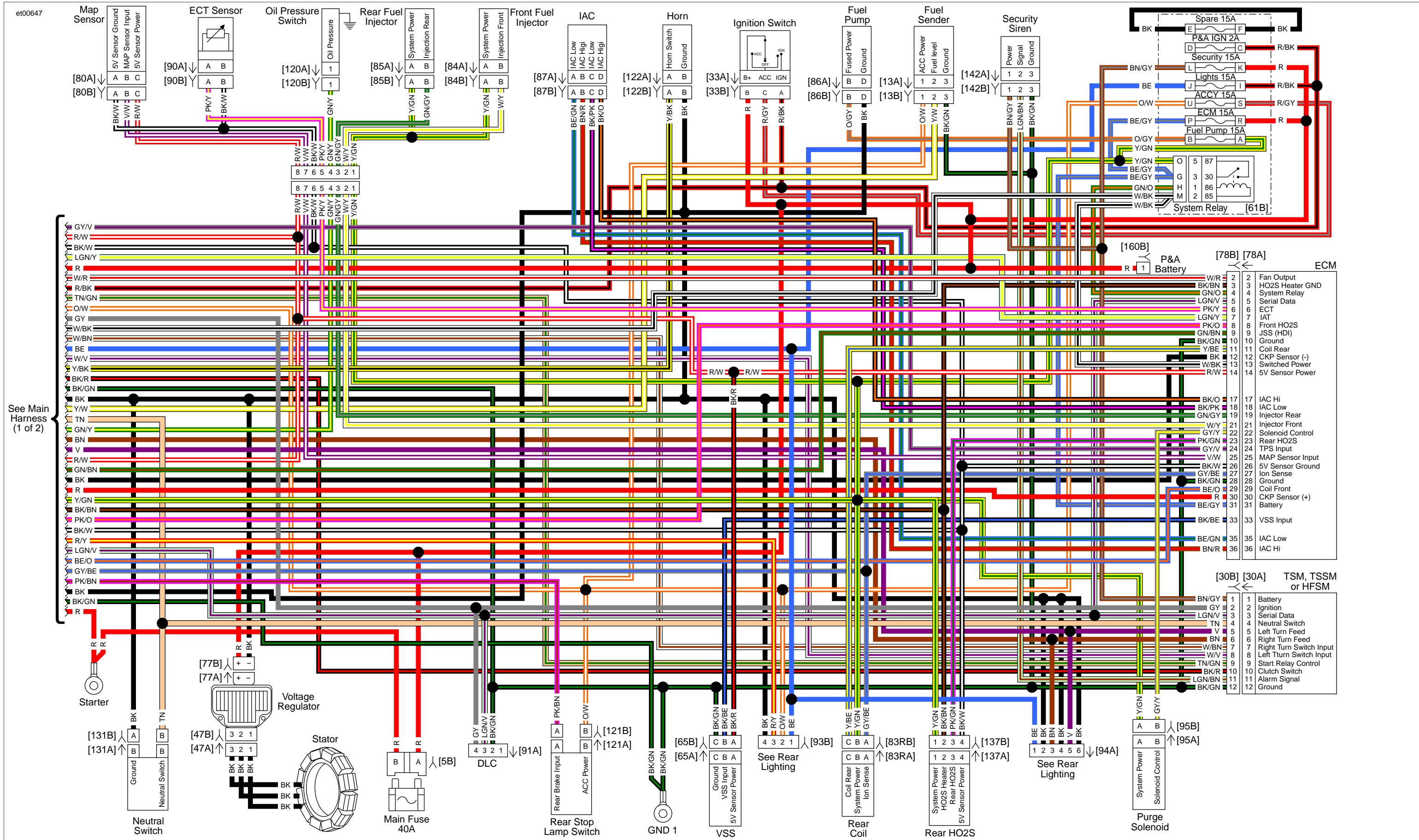
Main Harness (2 of 2): 2016 V-Rod
