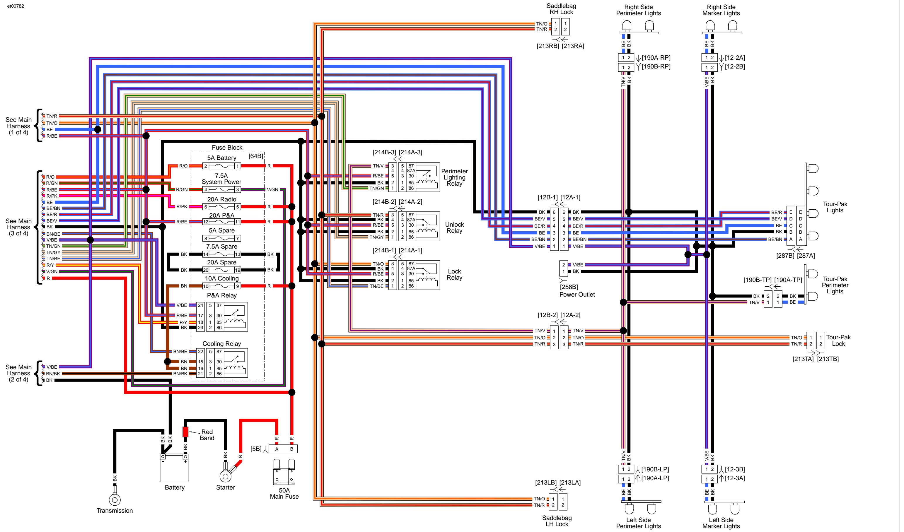
Main Harness (4 of 4): 2016 FLHTKSE
